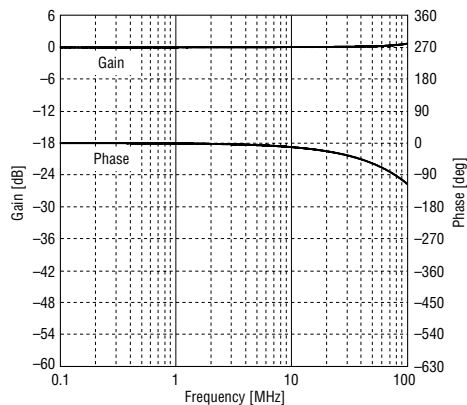
Figure 4. Gain and Phase characteristics (filter bypass mode)
