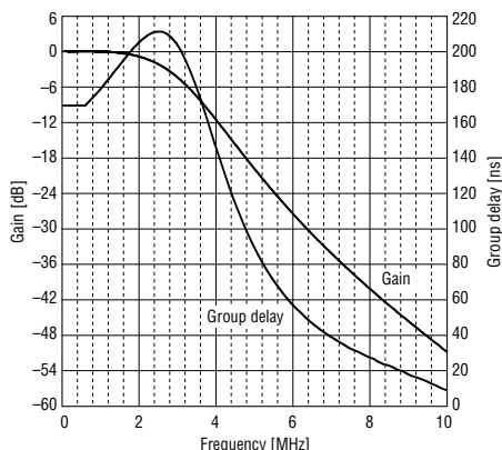
Figure 9. Gain and Group delay characteristics (half fc mode, FCDDATA = 10)
