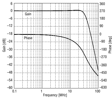
Figure 10. Gain and Phase characteristics (standard fc mode, FCDA = 227)
