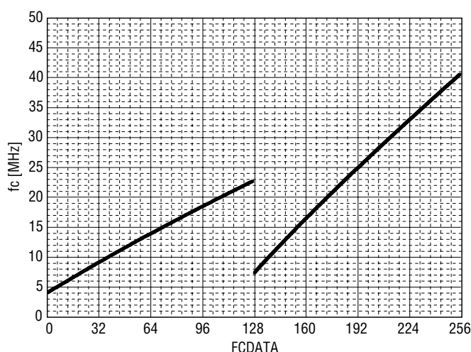
Figure 1. Cutoff frequency vs. FCDATA ( R_{ISET} = 1.8k\Omega )
