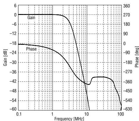
Figure 8. Gain and Phase characteristics (half fc mode, FCDDATA = 10)
