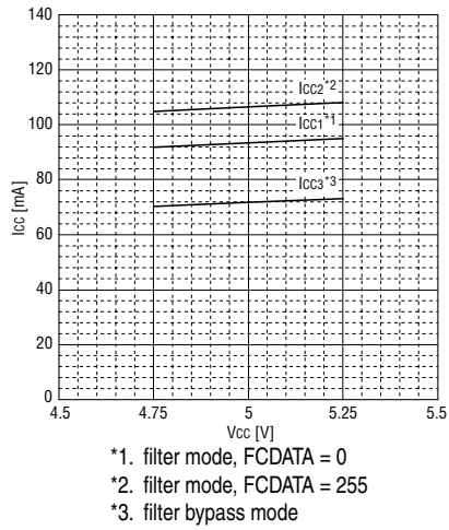
Figure 17. I_{CC1, 2, 3} vs. V_{CC}
