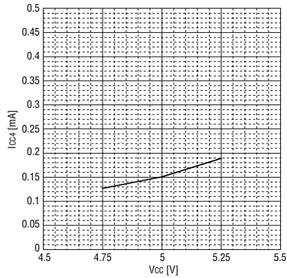
Figure 19. I_{CC4} vs. V_{CC}
