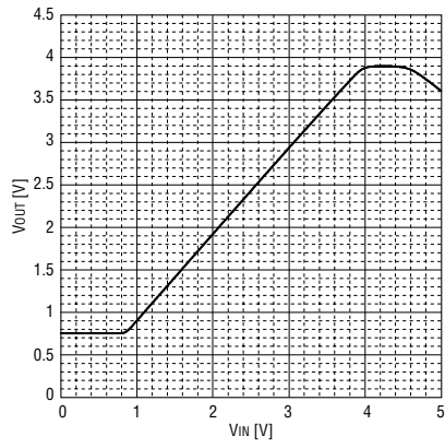
Figure 23. V_{IN} vs. V_{OUT} (filter mode, direct mode)
