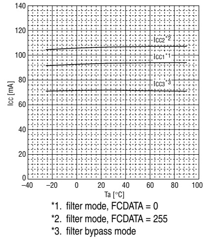
Figure 18. I_{CC1, 2, 3} vs. T_a
