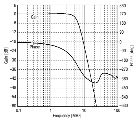
Figure 6. Gain and Phase characteristics (standard fc mode, FCDDATA = 10)
