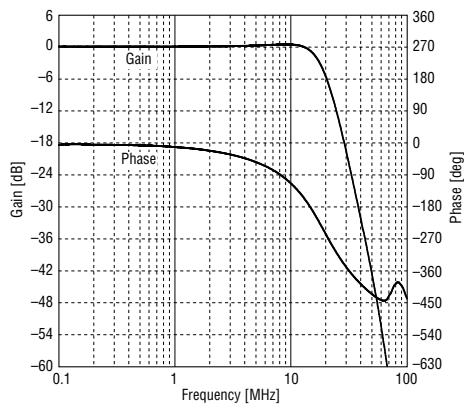
Figure 12. Gain and Phase characteristics (half fc mode, FCDA = 227)
