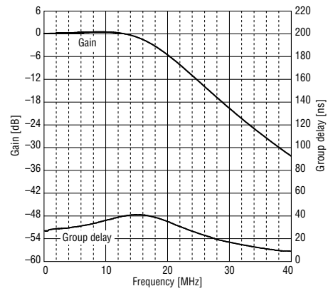
Figure 13. Gain and Group delay characteristics (half fc mode, FCDA = 227)
