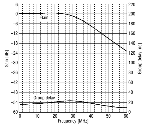
Figure 11. Gain and Group delay characteristics (standard fc mode, FCDA = 227)
