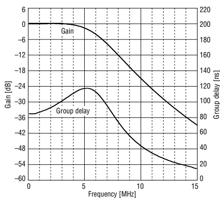
Figure 7. Gain and Group delay characteristics (standard fc mode, FCDDATA = 10)
