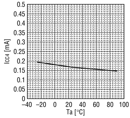
Figure 20. I_{CC4} vs. T_a
