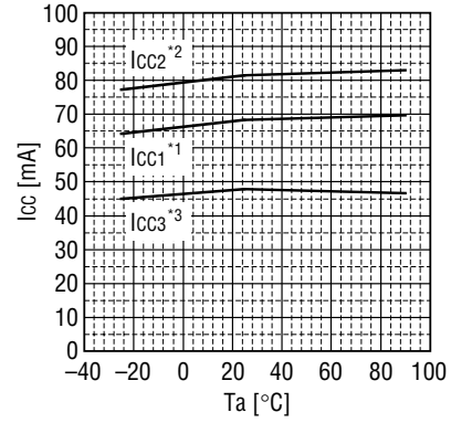
Figure 18. I_{CC1, 2, 3} vs. T_a
