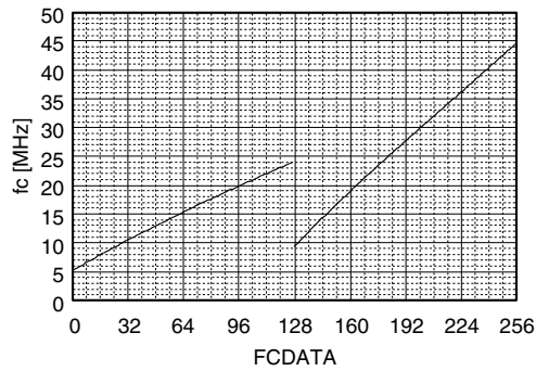
Figure 1. Cutoff frequency vs. FCDDATA ( R_{ISET} = 1.8k\Omega )
