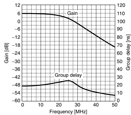
Figure 3. Gain and Group delay vs. Frequency characteristics (SD2 mode)
