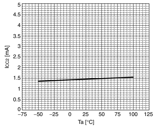
Figure 11. I_{CC2} vs. T_a (no signal input)
