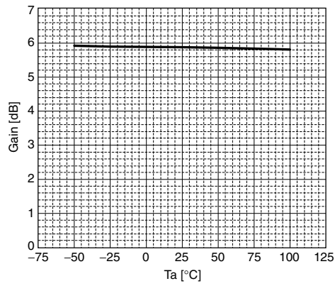
Figure 12. Gain vs. T_a ( f_{in} = 100\text{kHz} )
