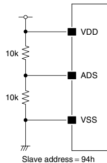
Figure 6. Slave address 94h setting
