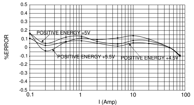
GRAPH 4 - Linearity PF=1, Supply=+5.5V, +5V, +4.5V
