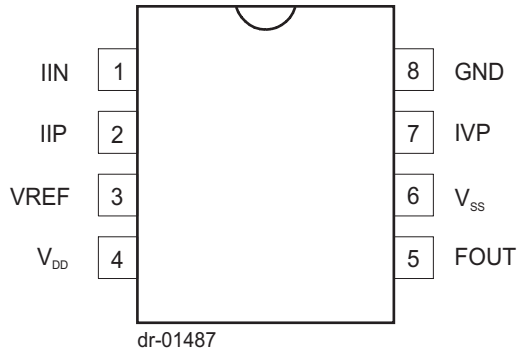
Figure 2: Pin connections: Package: PDIP8
