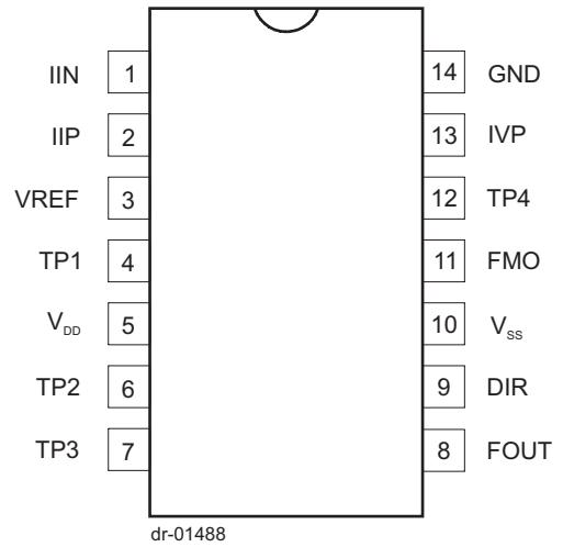
Figure 3: Pin connections: Package: PDIP14
