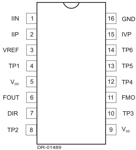
Figure 4: Pin connections: Package: SOIC16
