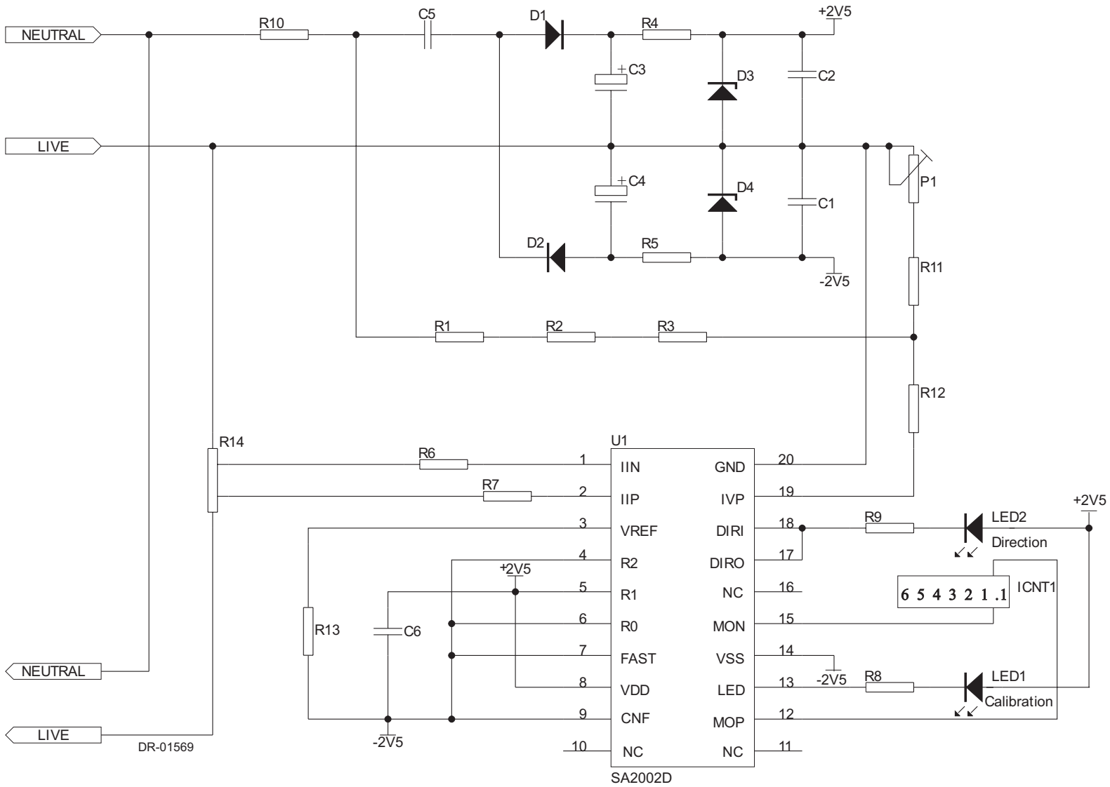
Figure 7: Application Circuit
