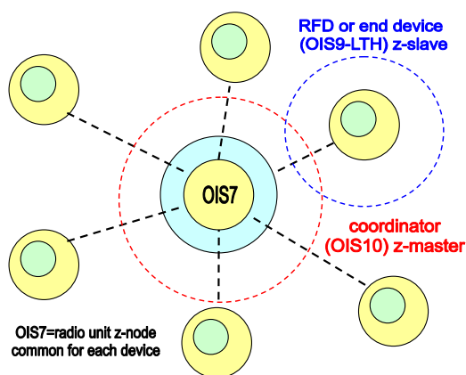
Figure 1 – Star network (1 coordinator and many RFD)
