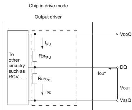
FIGURE 19 - OUTPUT DRIVER
