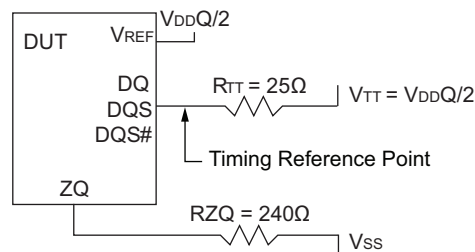
FIGURE 22 - REFERENCE OUTPUT LOAD FOR AC TIMING AND OUTPUT SLEW RATE
