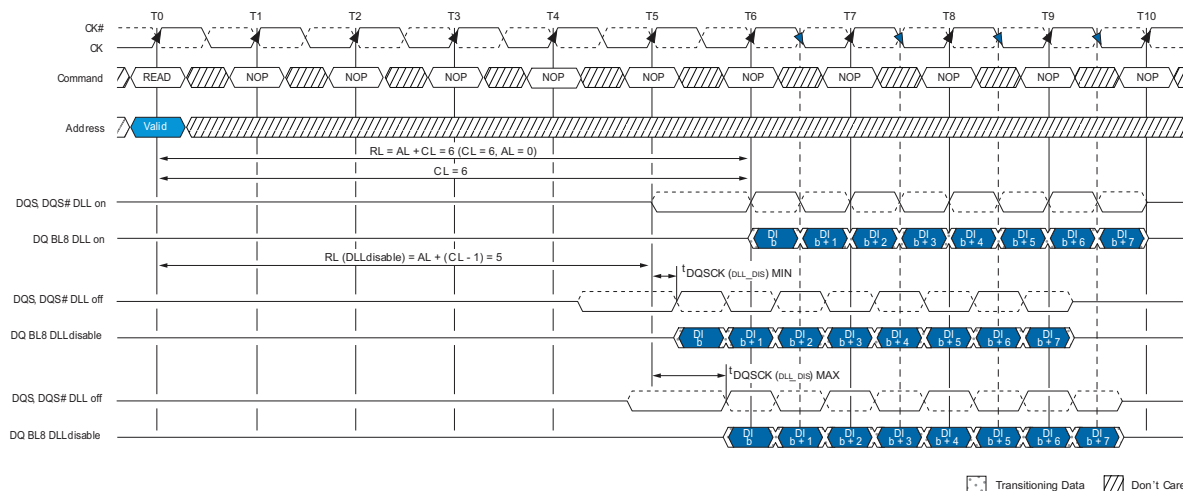
FIGURE 36 - DLL DISABLE t_{DQSK} TIMING
