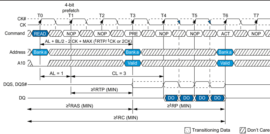
FIGURE 44 - READ-TO-PRECHARGE – BL = 4
