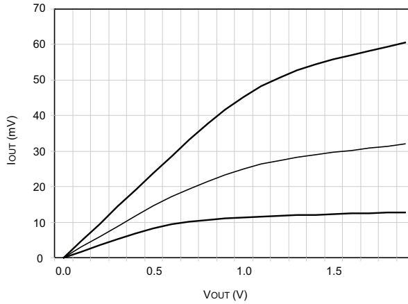
FIGURE 12 - REDUCED STRENGTH PULL DOWN CHARACTERISTICS
