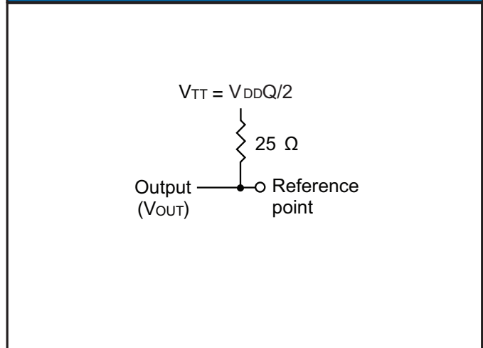
FIGURE 9 - OUTPUT SLEW RATE LOAD
