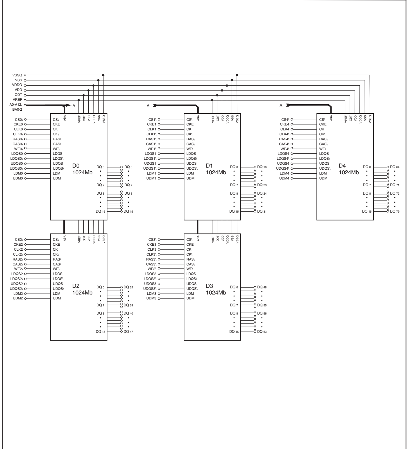
FIGURE 2F - FUNCTIONAL BLOCK DIAGRAM
