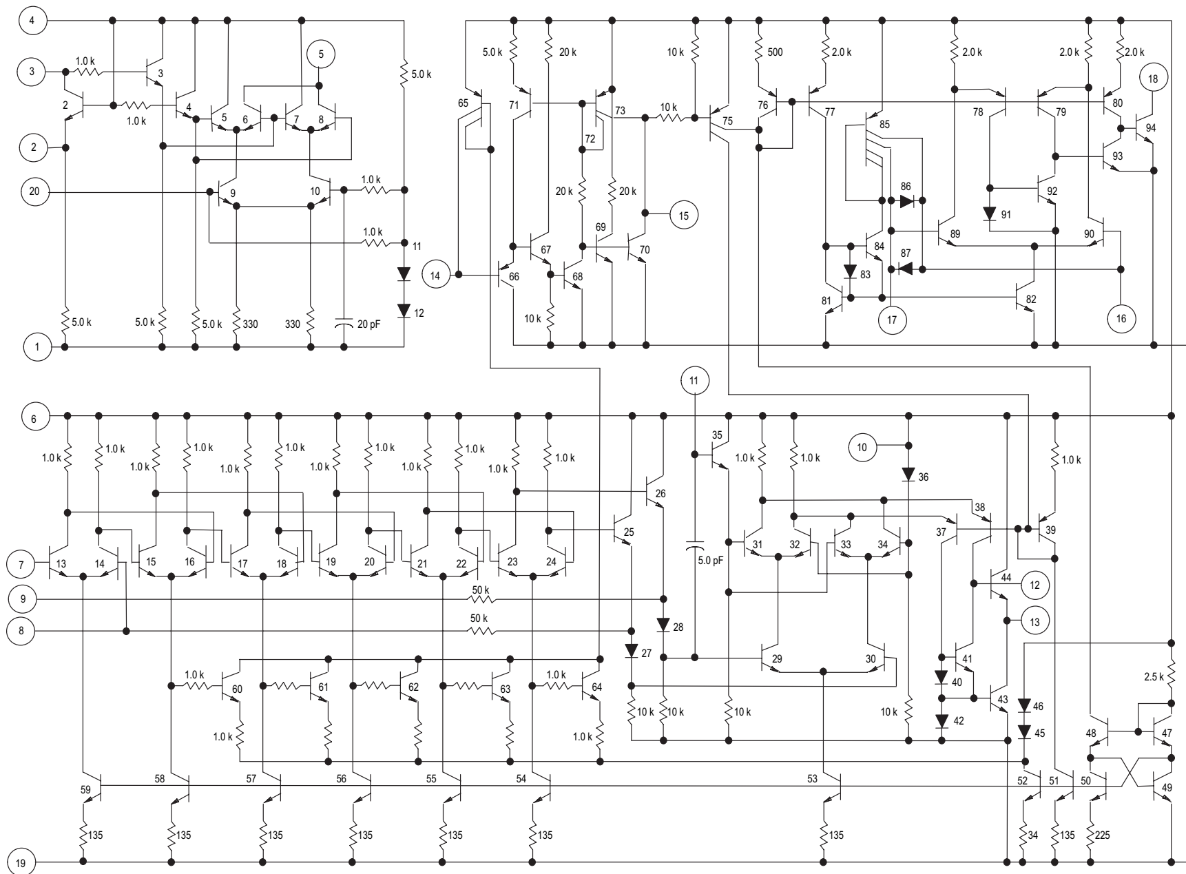
Figure 7. Internal Schematic
