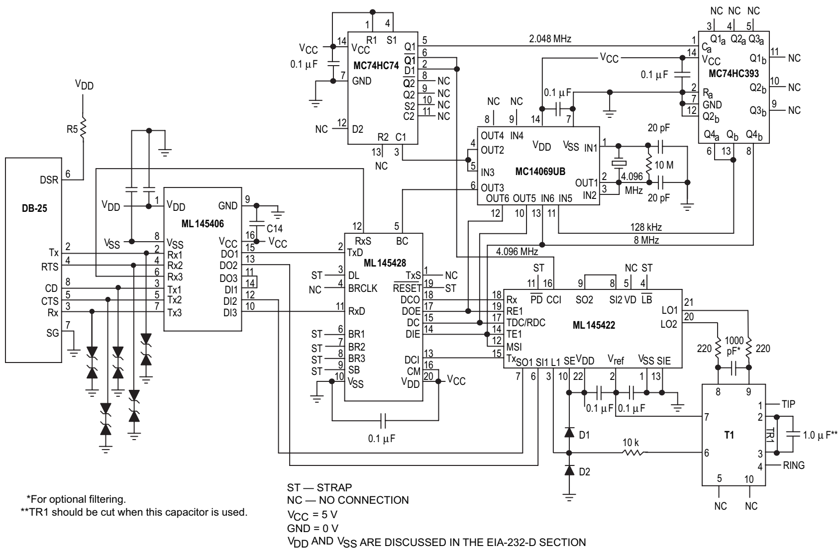
Figure 7. 80-kbps Limited Distance Modem with EIA 232-E Interface (Master)
