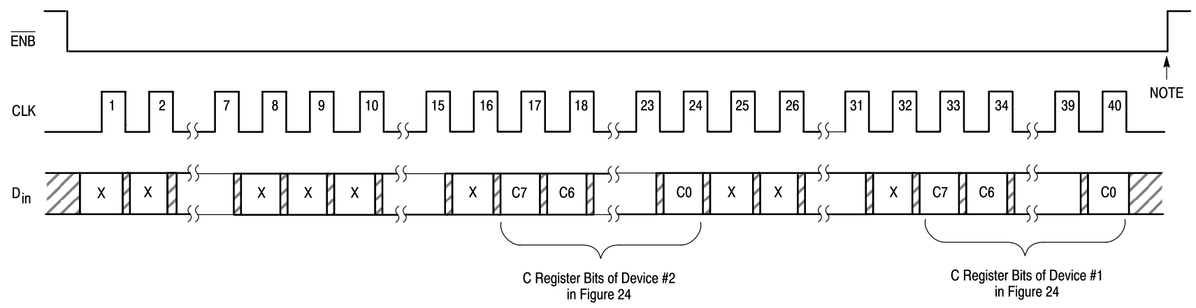
Figure 25. Accessing the C Registers of Two Cascading ML145170 Devices
