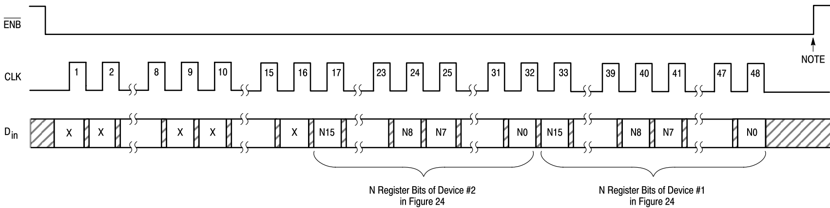
Figure 27. Accessing the N Registers of Two Cascaded ML145170 Devices
