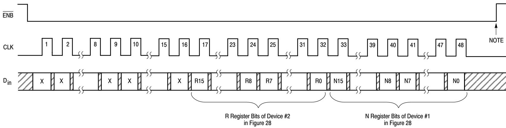
Figure 31. Accessing the R and N Registers of Two Different Device Types
