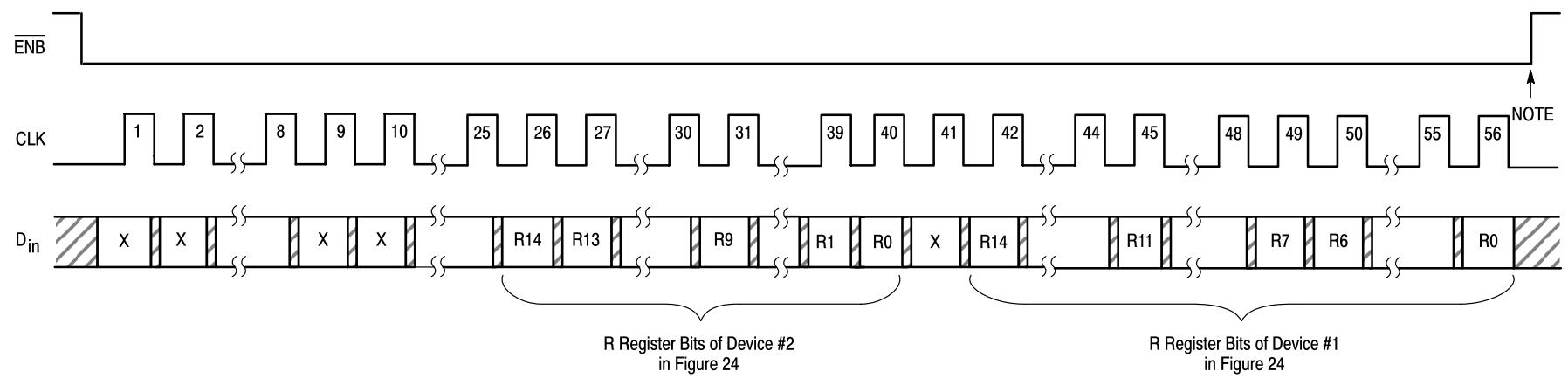
Figure 26. Accessing the R Registers of Two Cascading ML145170 Devices
