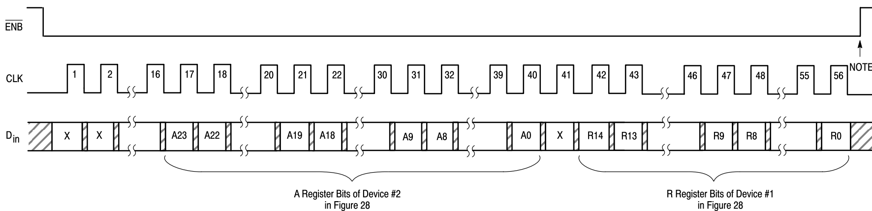
Figure 30. Accessing the A and R Registers of Two Different Device Types
