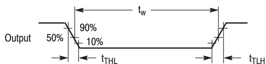
Figure 11. Switching Waveform
