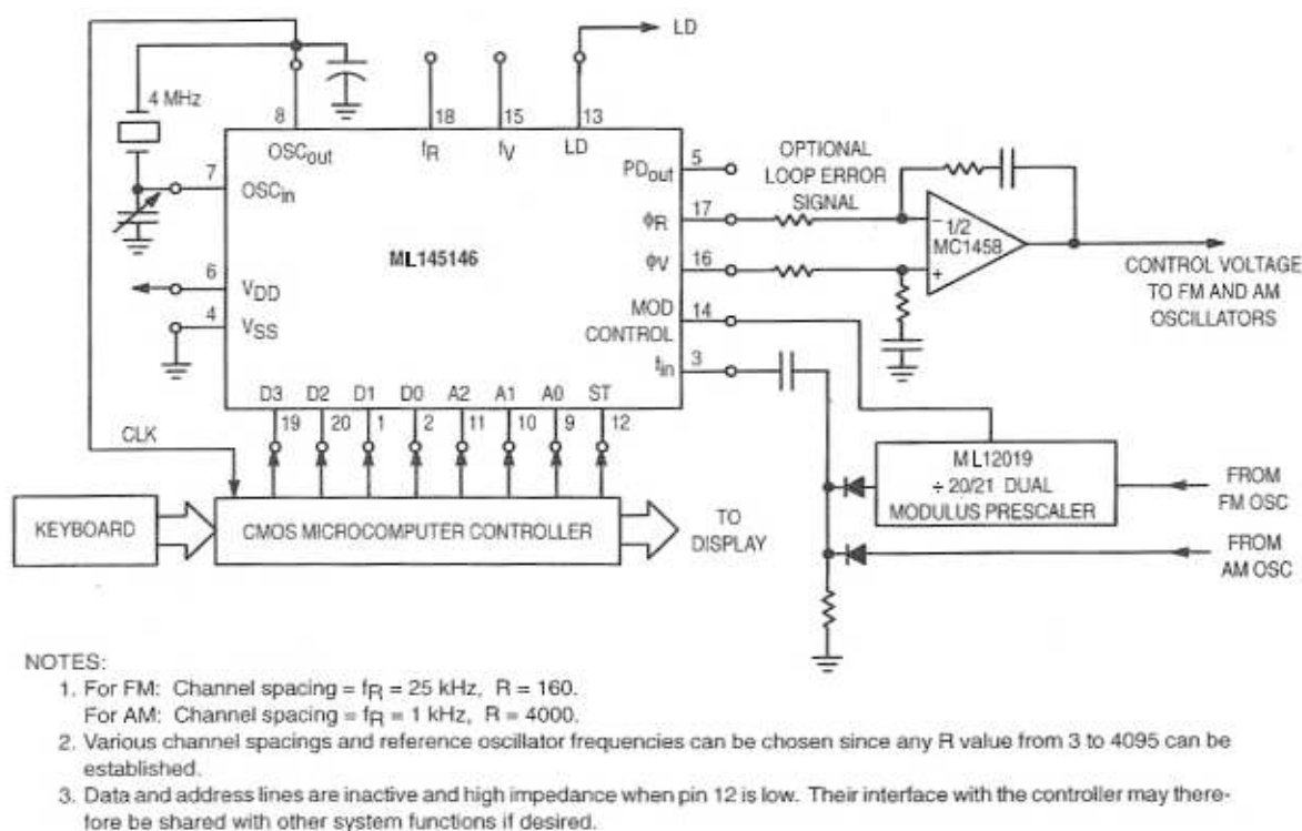
Figure 12. FM/AM Broadcast Radio Synthesizer
