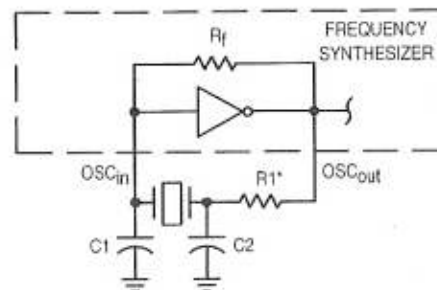
Figure 8. Pierce Crystal Oscillator Circuit
