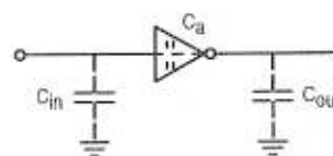
Figure 9. Parasitic Capacitances of the Amplifier
