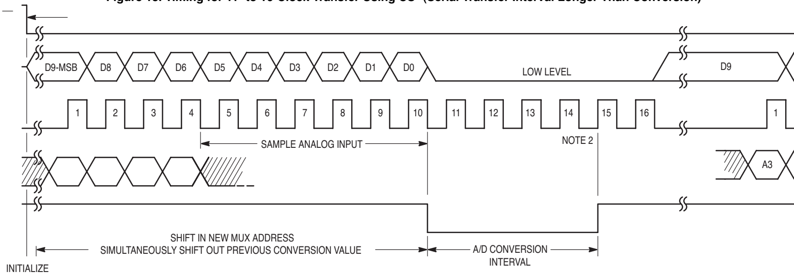
Figure 14. Timing for 16-Clock Transfer Not Using \overline{CS}^* (Serial Transfer Interval Longer Than Conversion)
