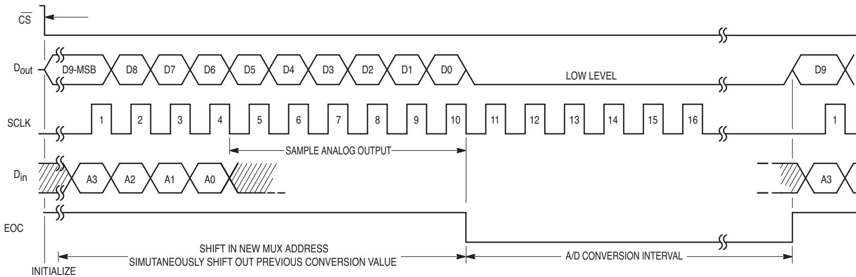
Figure 12. Timing for 16-Clock Transfer Not Using \overline{CS}^* (Serial Transfer Interval Shorter than Conversion)
