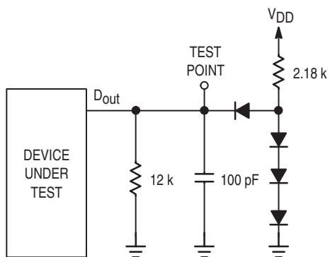
Figure 7. Test Circuit
