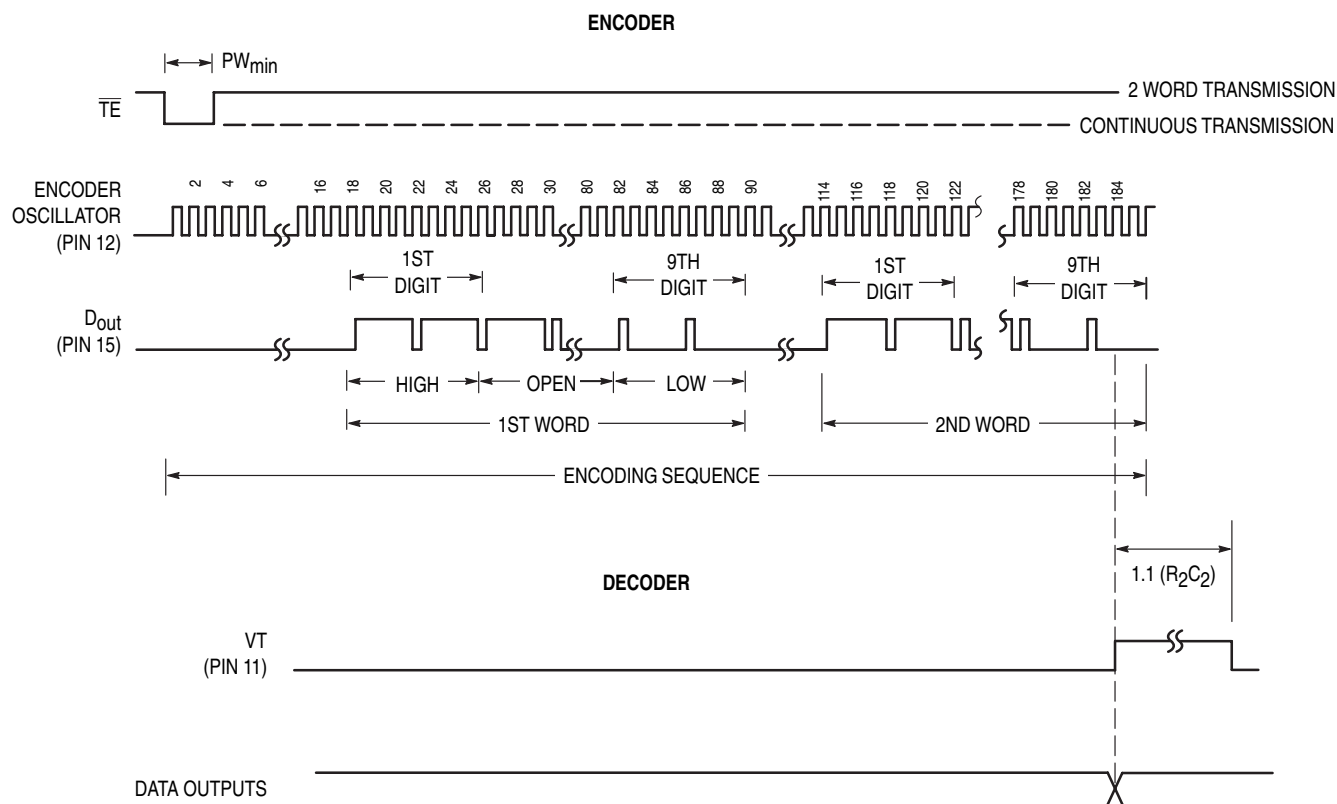
Figure 10. Timing Diagram
