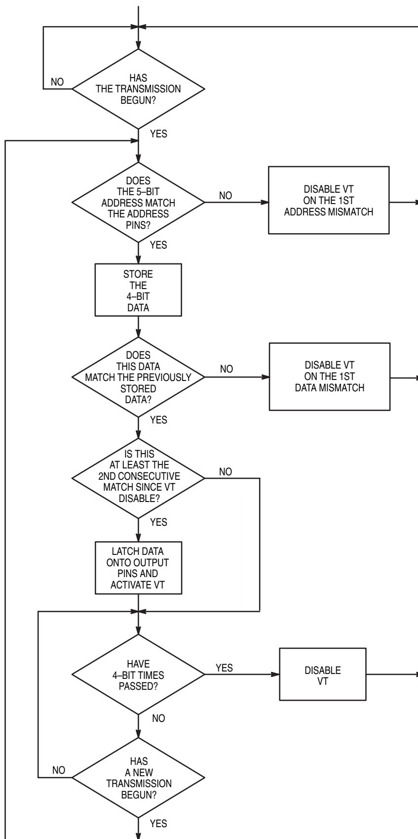
Figure 13. ML145027 Flowchart
