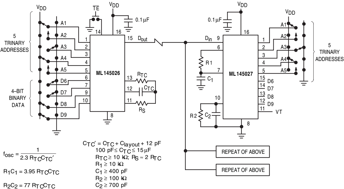
Example R/C Values (All Resistors and Capacitors are ± 5%)
