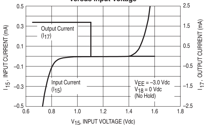
Figure 15. Data Slicer Input/Output Currents versus Input Voltage
