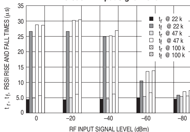
Figure 25. RSSI Output Rise and Fall Times versus RF Input Signal Level
