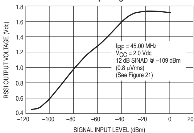
Figure 22. RSSI Output Voltage versus Input Signal Level
