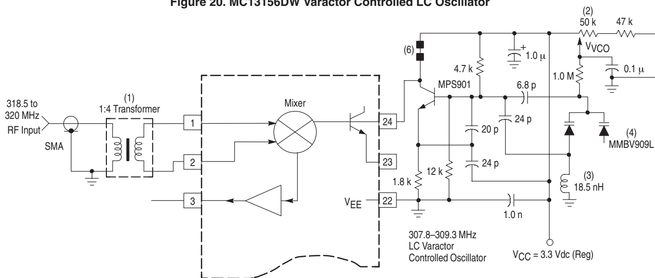
Figure 20. MC13156DW Varactor Controlled LC Oscillator
