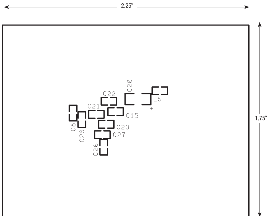
Figure 12. ML13146 Evaluation PCB Solder Side
