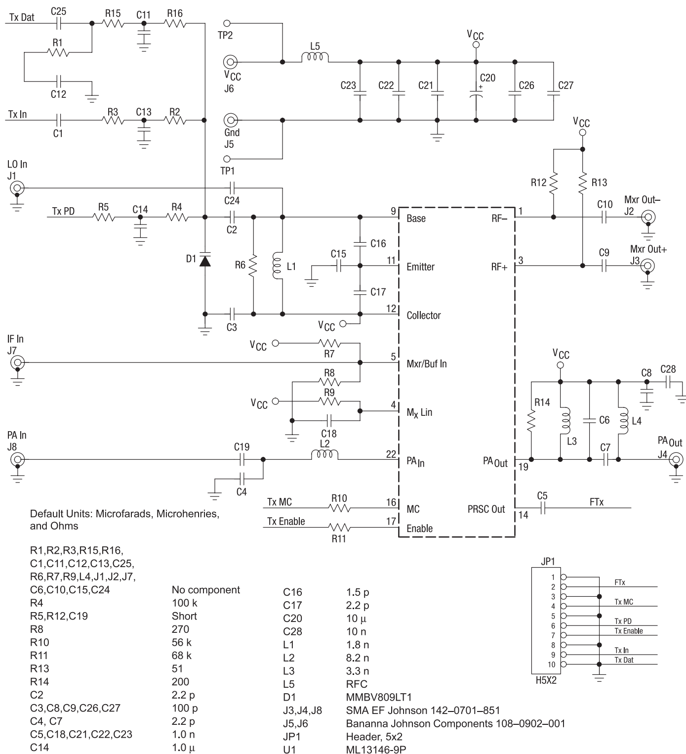
Figure 9. Evaluation PCB Schematic
