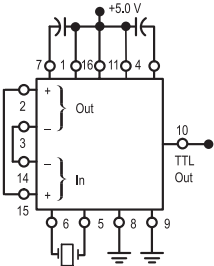
Figure 3. M TTL Output
