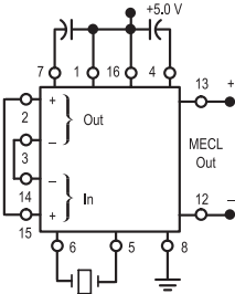
Figure 4. MECL Output (+5.0 V Supply)
