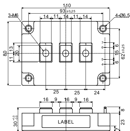
PDMB400B12
