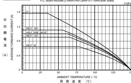
平均順電流一周周囲温度定格 AVERAGE FORWARD CURRENT VS. AMBIENT TEMPERATURE P.C. Board mounted (L=8mm, Print Land=10×10mm, Both Sides)
