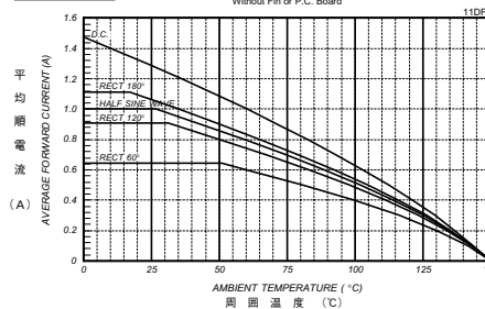
平均順電流一周周囲温度定格 AVERAGE FORWARD CURRENT VS. AMBIENT TEMPERATURE Without Fin or P.C. Board
