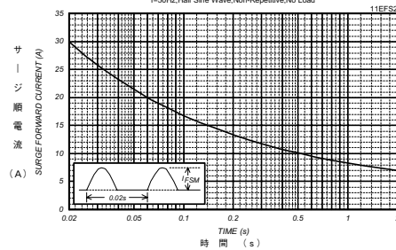
サージ順電流定格 SURGE CURRENT RATINGS 1=50Hz Half Sine Wave, Non-Repetitive, No Load
