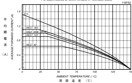
平均順電流一周囲温度定格 AVERAGE FORWARD CURRENT VS. AMBIENT TEMPERATURE P.C. Board mounted (L=3mm, Print Land=5×5mm, Both Sides)
