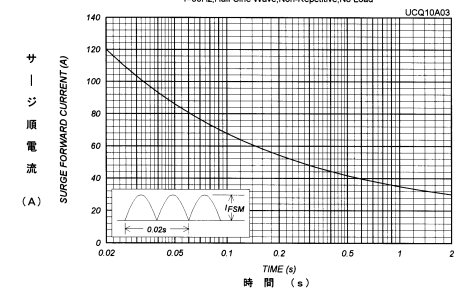
FIG.6 サージ順電流定格 SURGE CURRENT RATINGS f=50Hz Half Sine Wave, Non-Repetitive, No Load
