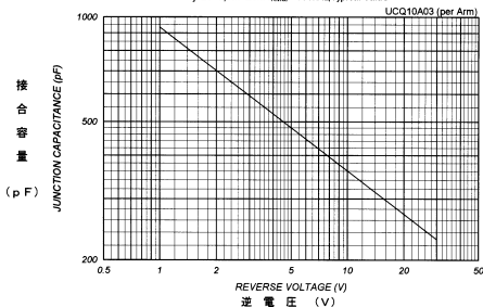
FIG.7 接合容量特性 JUNCTION CAPACITANCE VS. REVERSE VOLTAGE Tj=25°C, V m =20V RRM , f=100kHz, Typical Value
