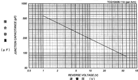
接合容量特性 JUNCTION CAPACITANCE VS. REVERSE VOLTAGE
