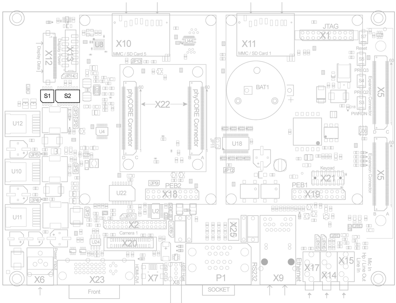
Figure 43: Boot Mode Selection Switches S1 and S2
