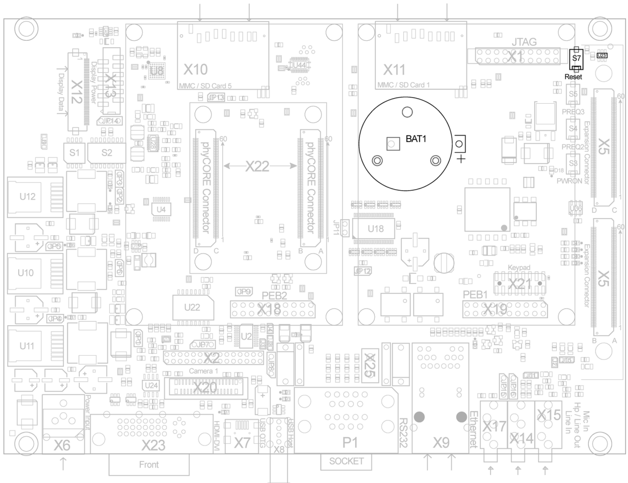
Figure 44: System Reset Button S7
