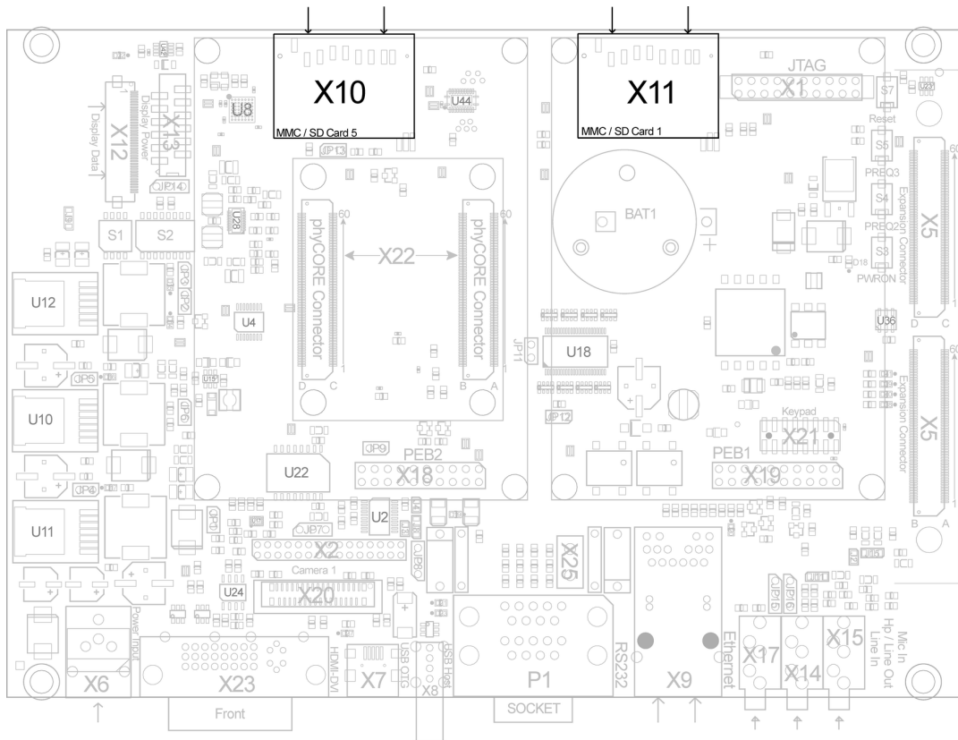
Figure 41: Components supporting the SD / MM Card interfaces at connector X10 and X11 (top view)
