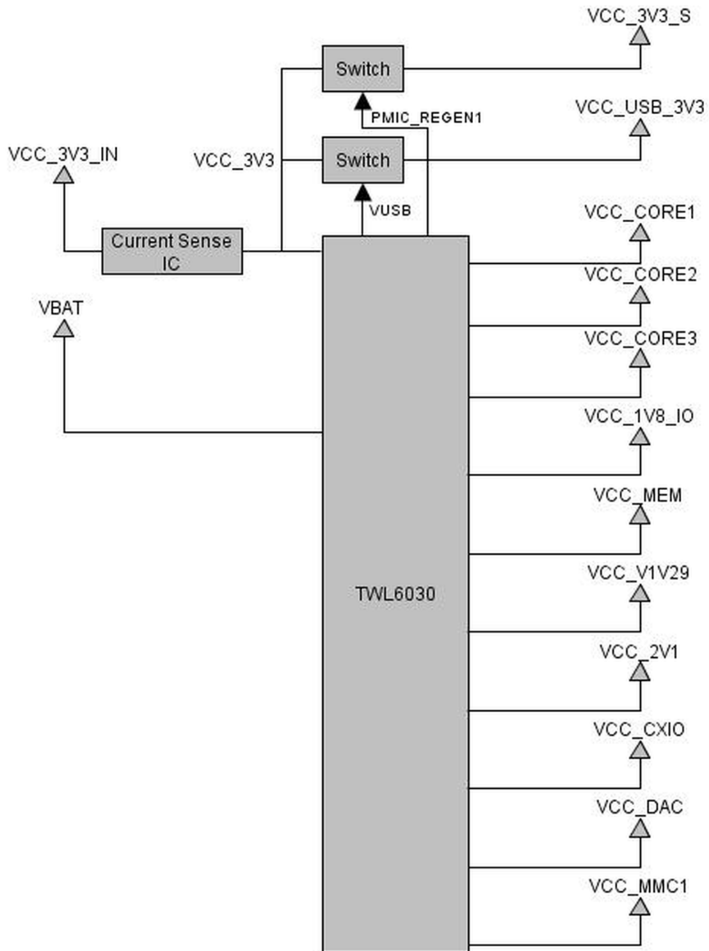
Figure 8: Power Supply Diagram
