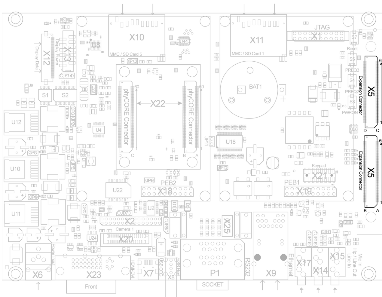
Figure 47: Expansion Connector X5
