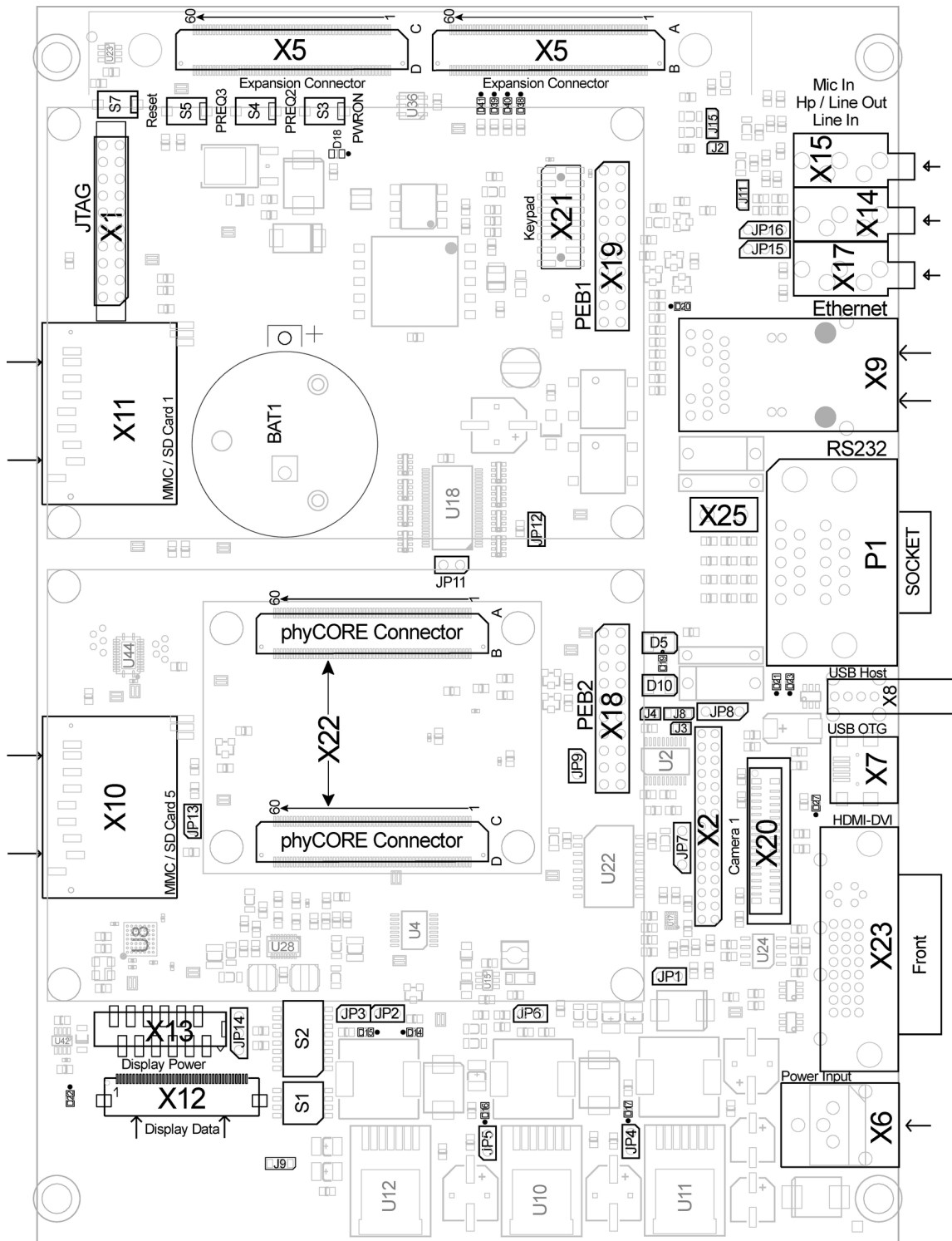
Figure 15: phyCORE-OMAP44xx Carrier Board Overview of Connectors, LEDs and Buttons (top view)
