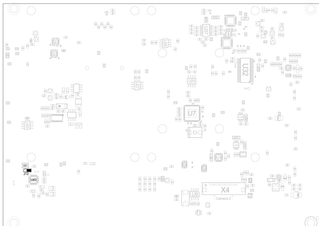
Figure 34: Components supporting the Audio Interface at connectors X5, X14, X15 and X17 (bottom view)
