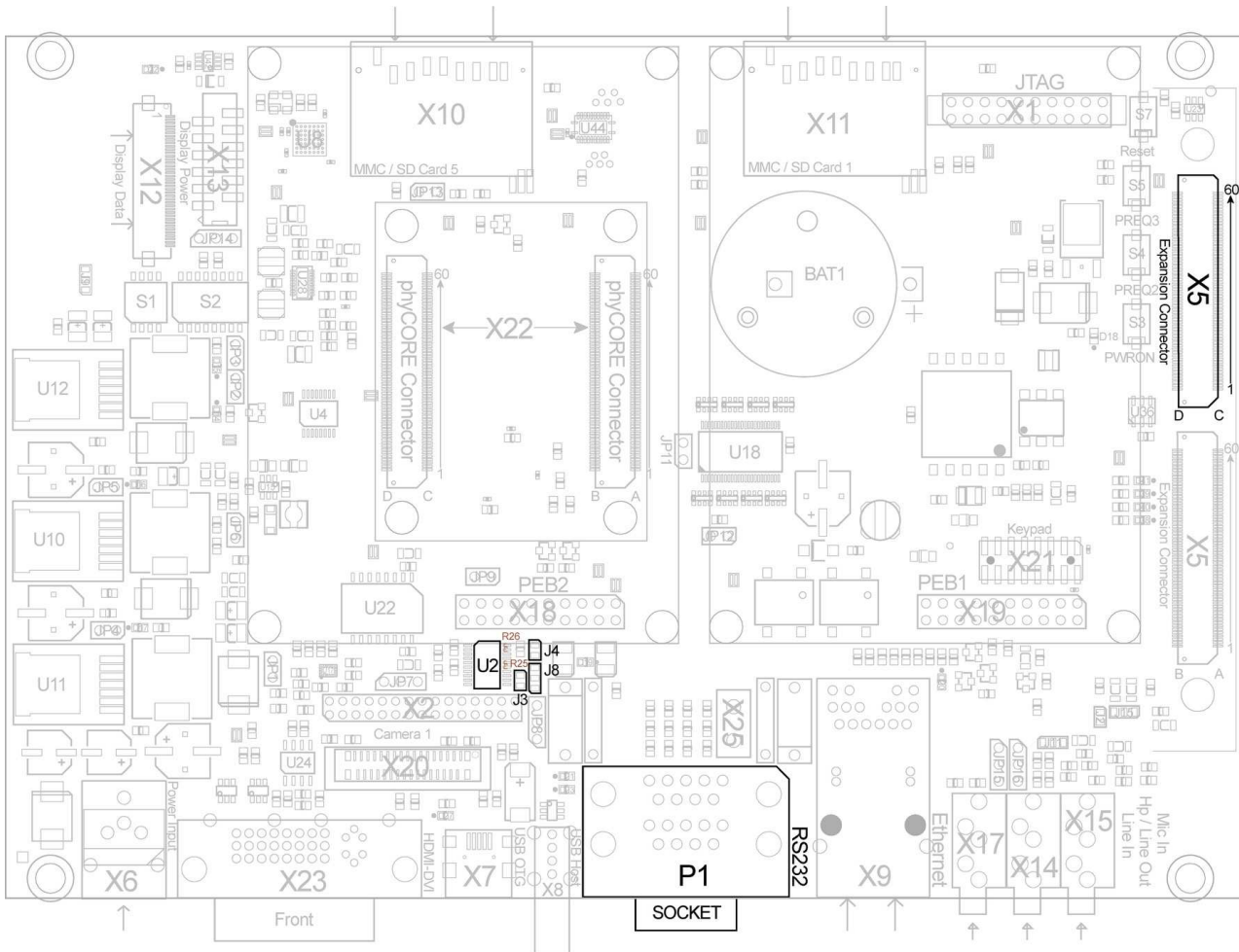
Figure 23: RS-232 Interface Connectors (P1, X5) and Jumpers
