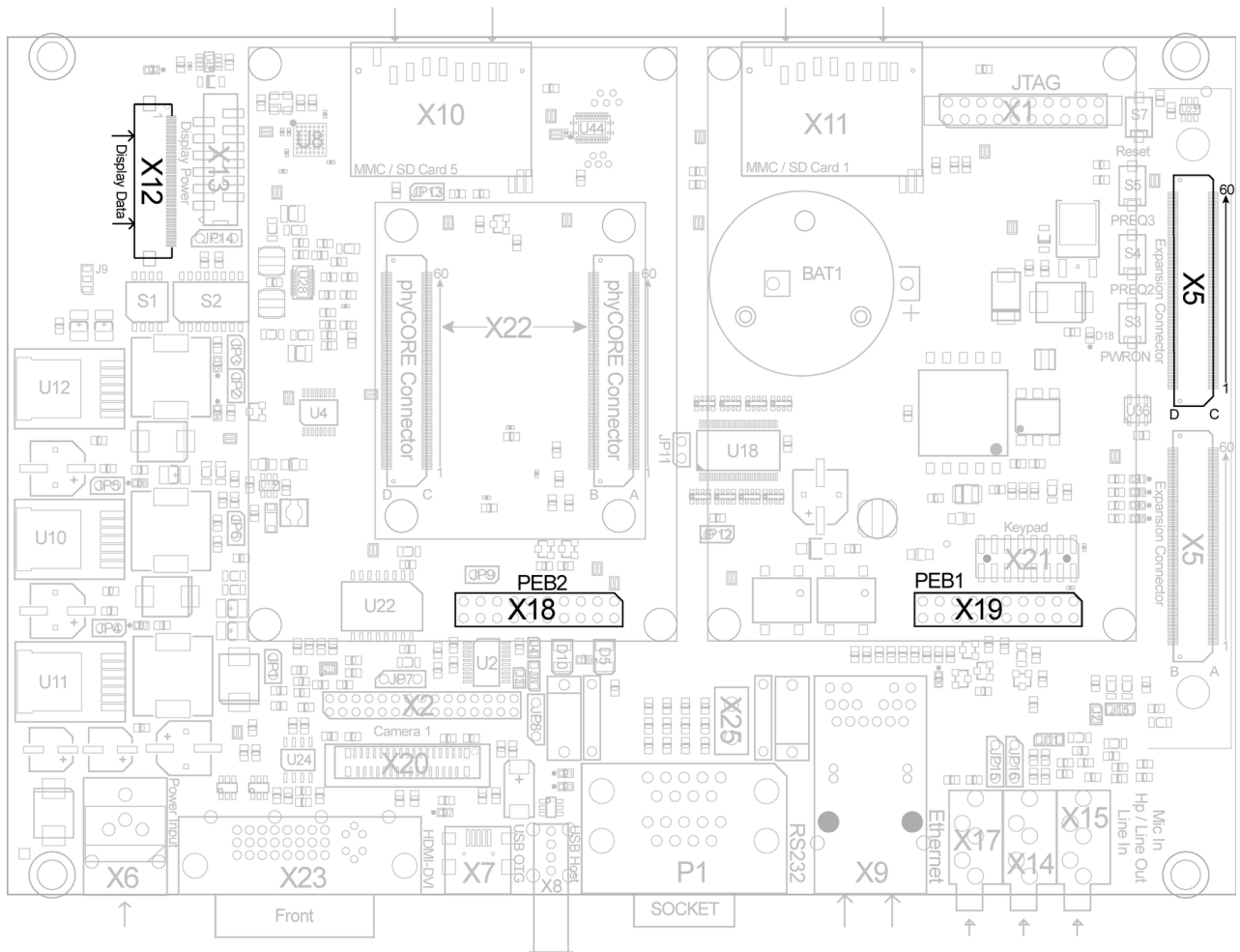
Figure 37: SPI Connectivity
