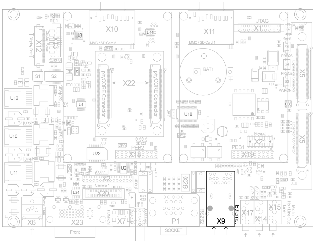
Figure 25: Ethernet Interface at Connector X9
