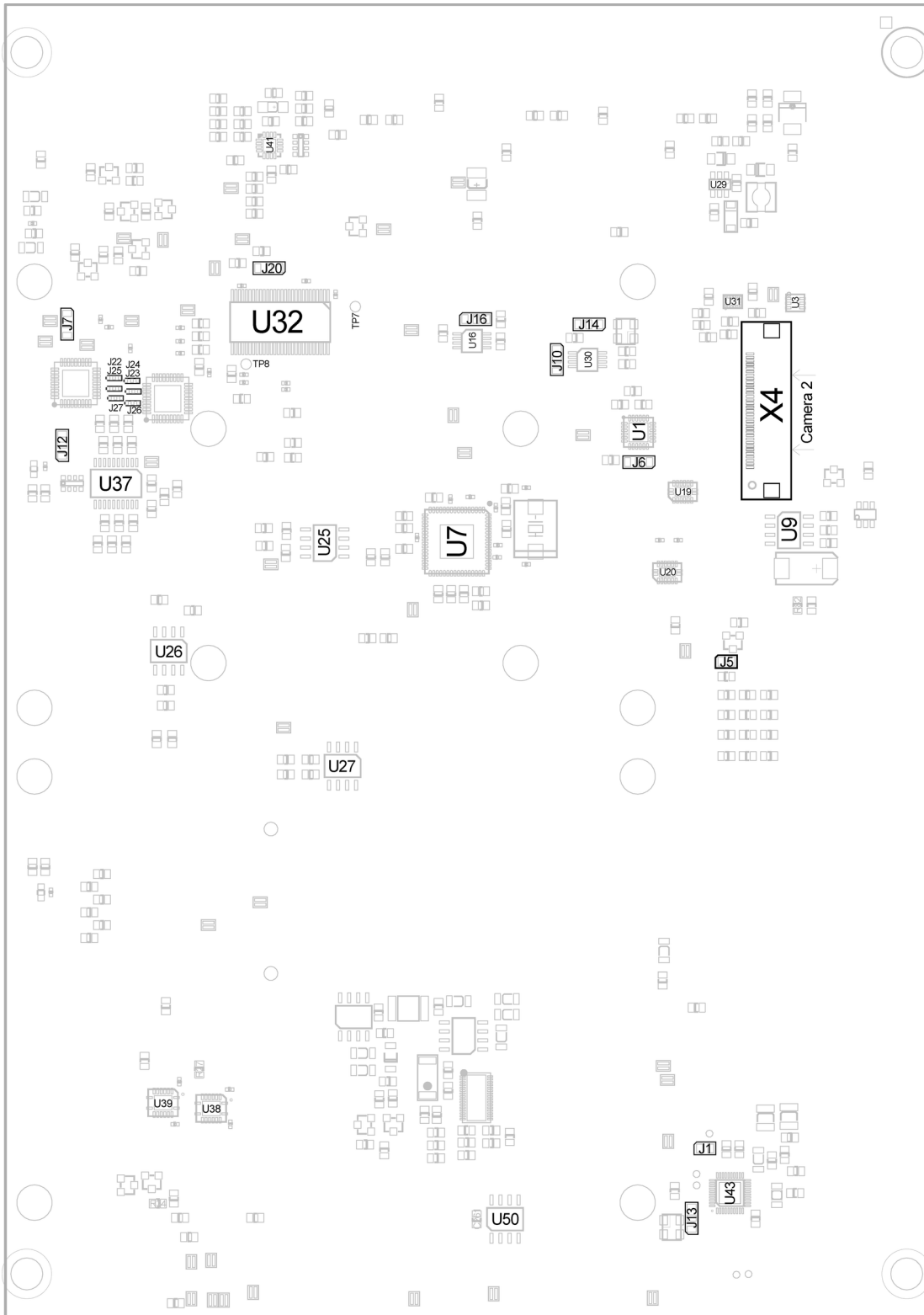
Figure 16: phyCORE-OMAP44xx Carrier Board Overview of Connectors, LEDs and Buttons (bottom view)
