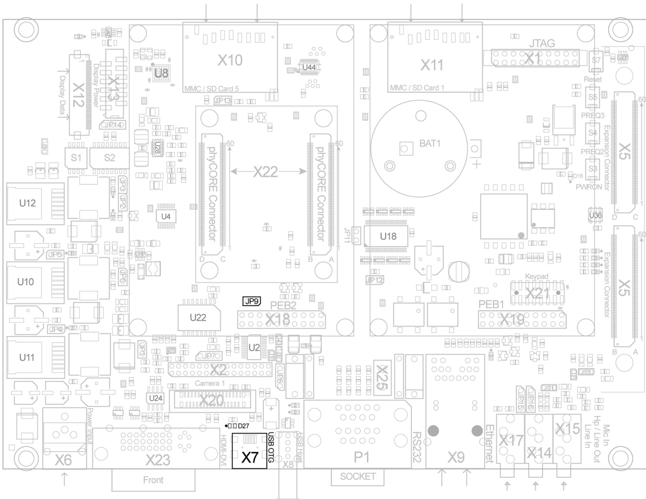
Figure 27: USB OTG Interface at Connector X7
