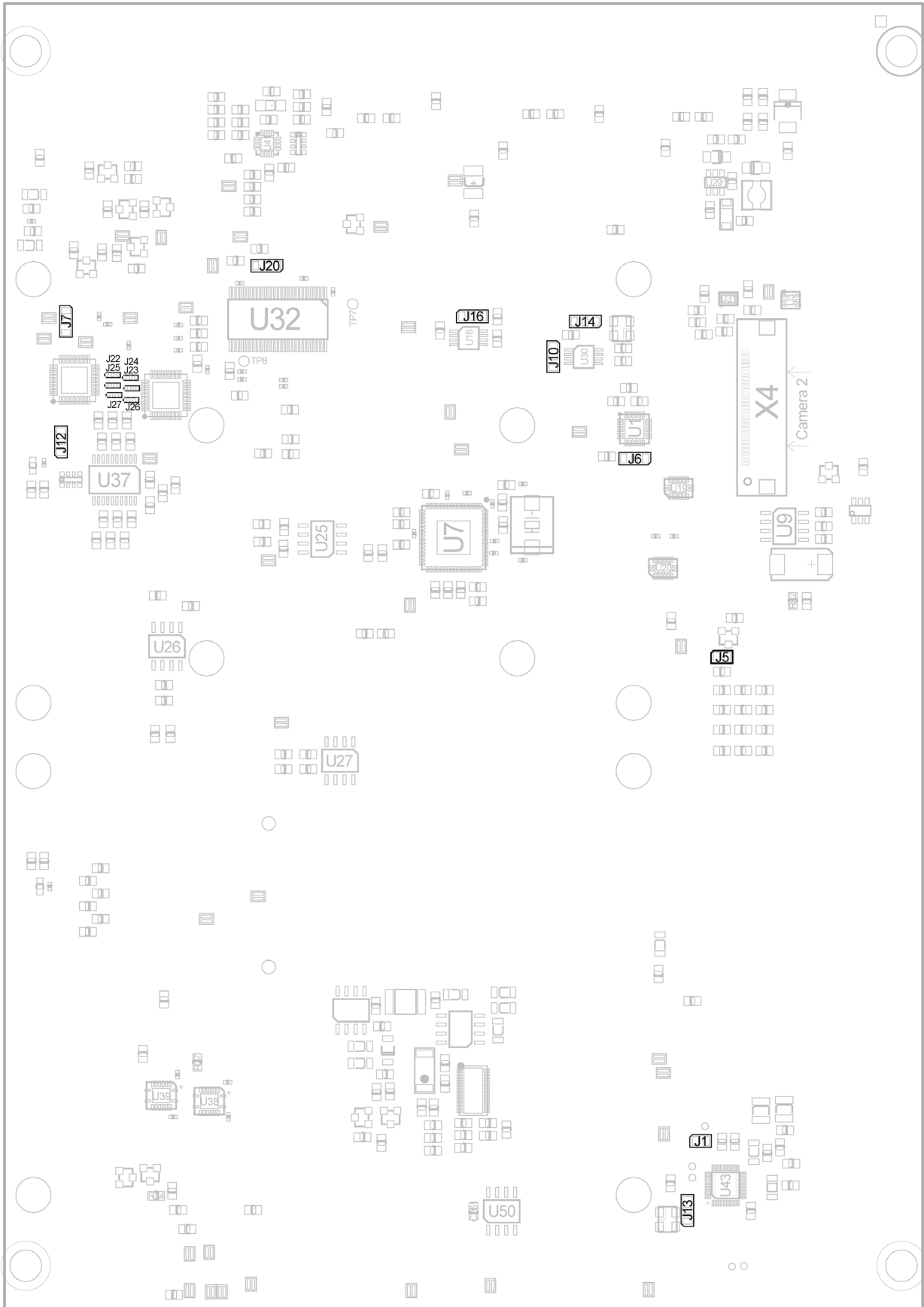
Figure 19: phyCORE-OMAP44xx Carrier Board Jumper Locations (bottom view)
