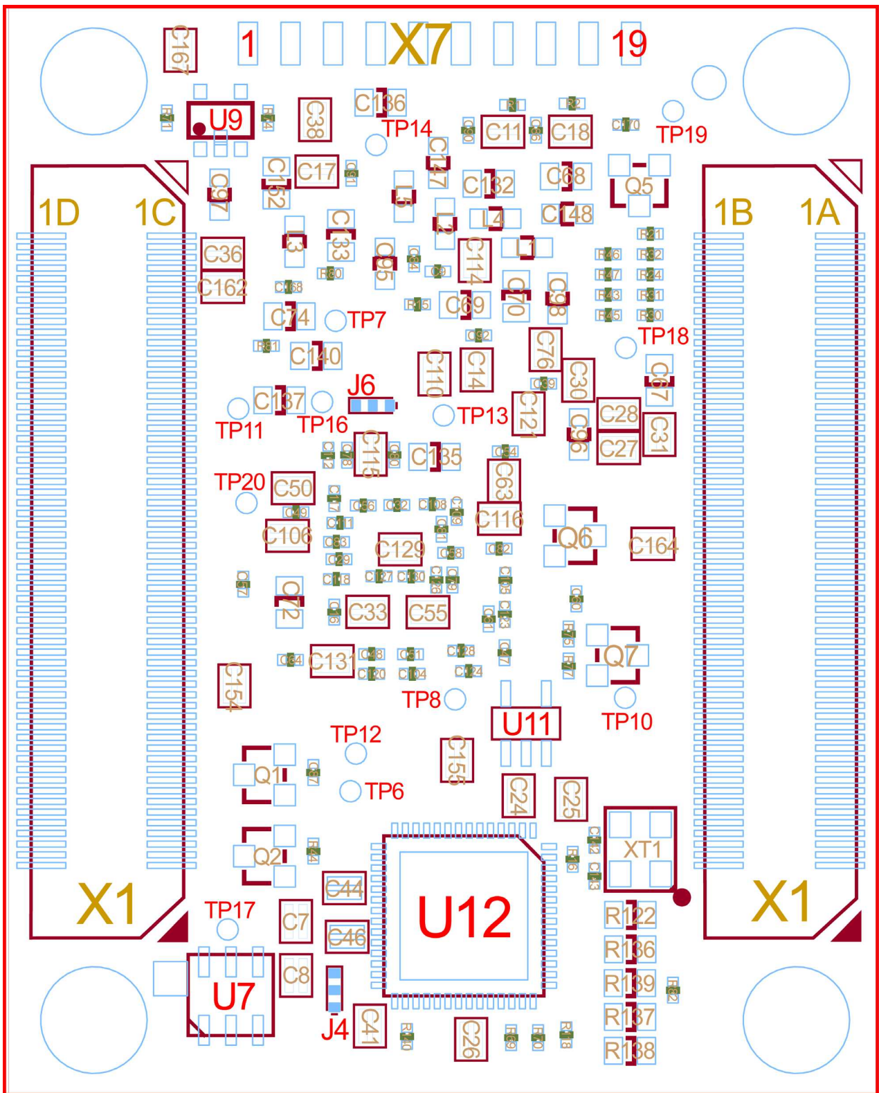
Figure 14: phyCORE-OMAP44xx Component Placement (bottom view)
