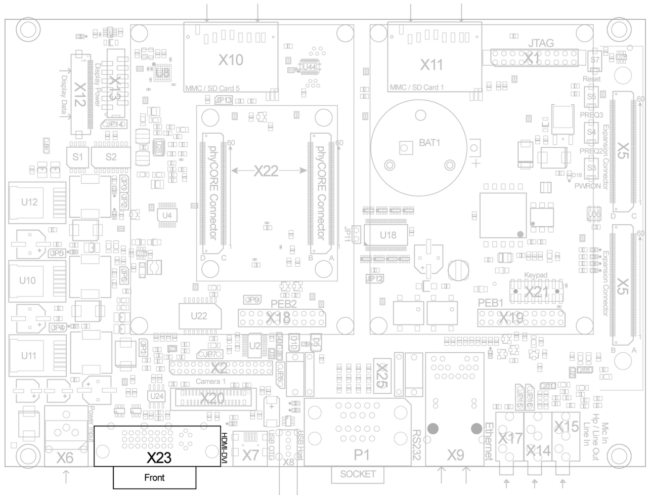
Figure 30: HDMI - DVI Connectivity (X23)
