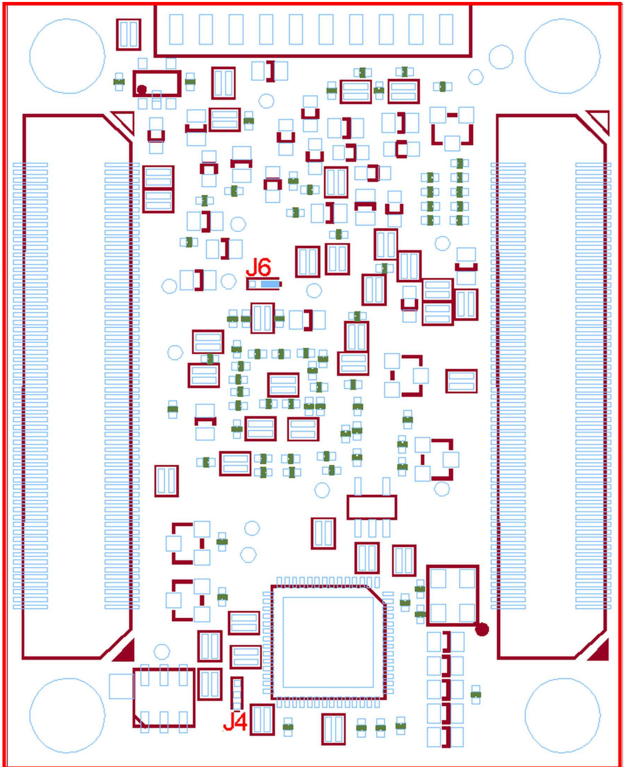
Figure 7: Jumper Locations (bottom view)
