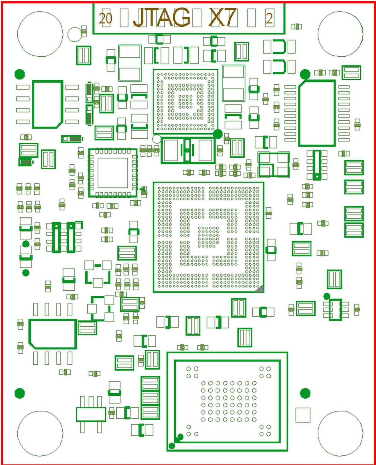
Figure 9: JTAG Interface at X7 (top view)
