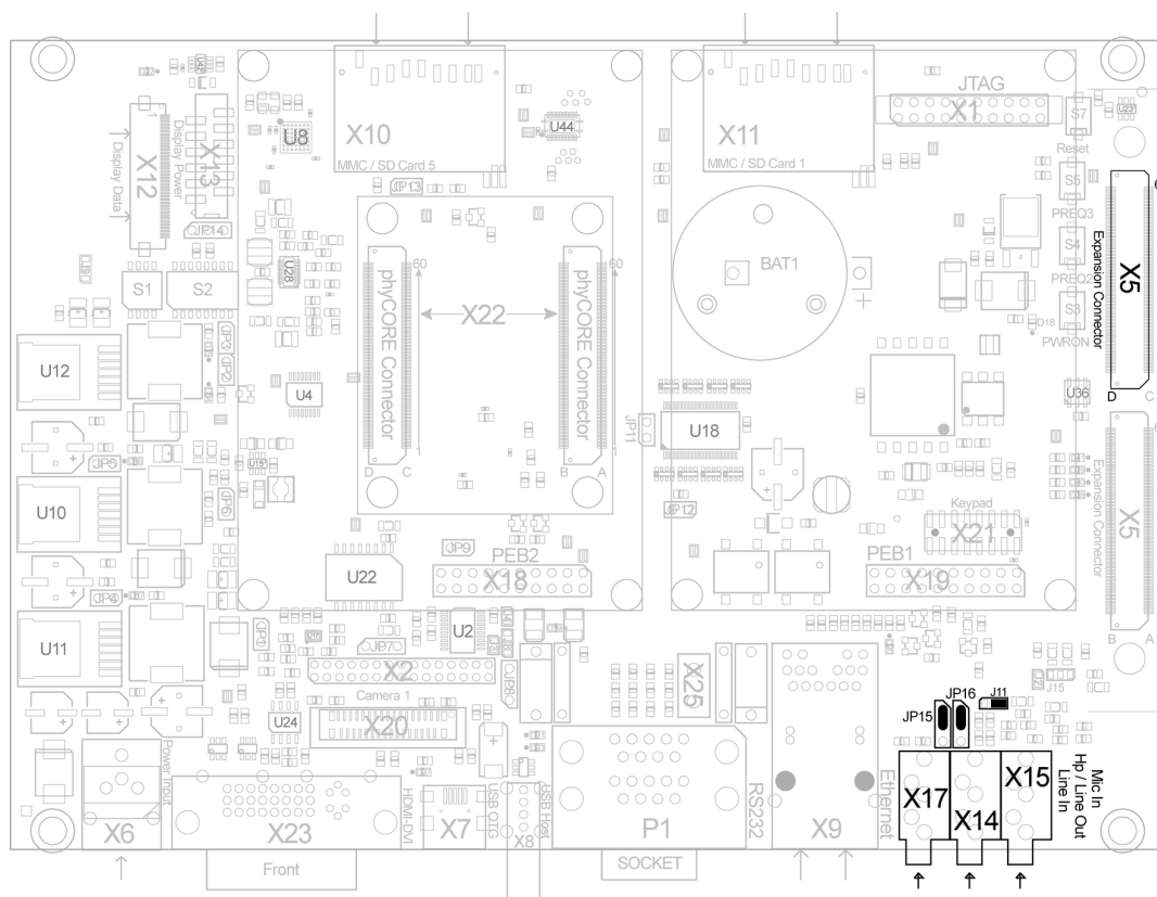
Figure 33: Components supporting the Audio Interface at connectors X5, X14, X15 and X17 (top view)
