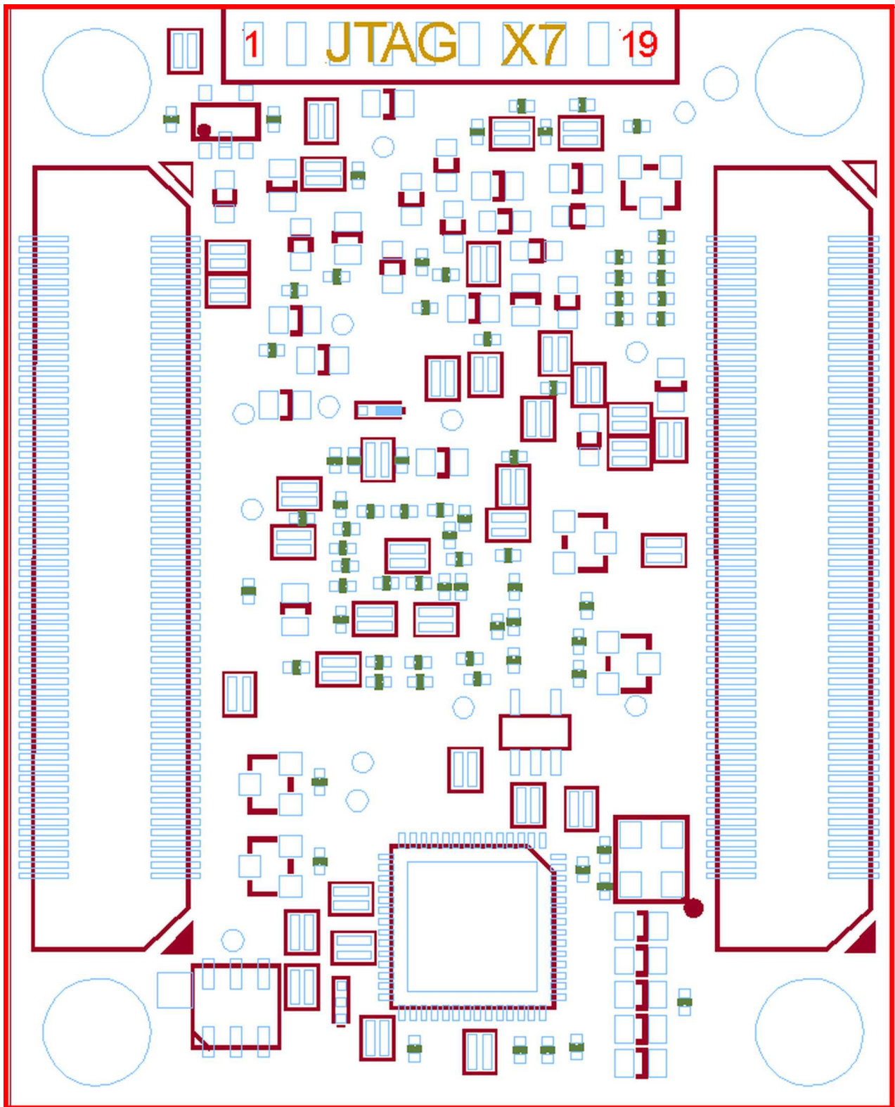
Figure 10: JTAG Interface at X7 (bottom view)
