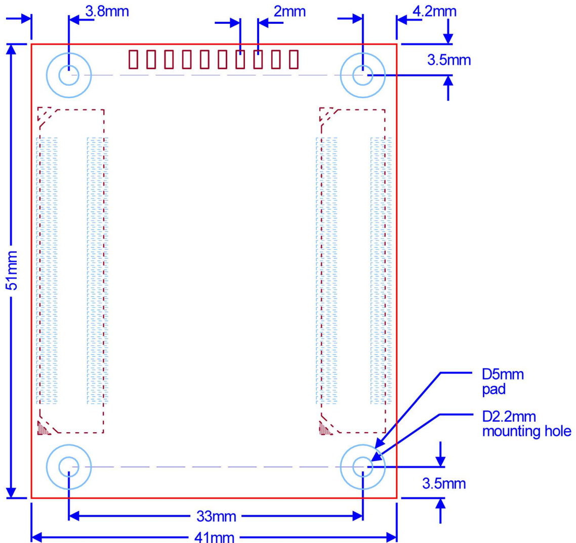
Figure 11: Physical Dimensions
