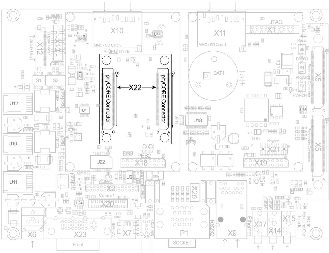
Figure 20: phyCORE-OMAP44xx SOM Connectivity to the Carrier Board
