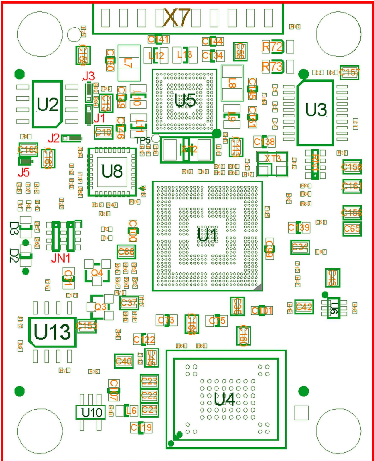
Figure 13: phyCORE-OMAP44xx Component Placement (top view)
