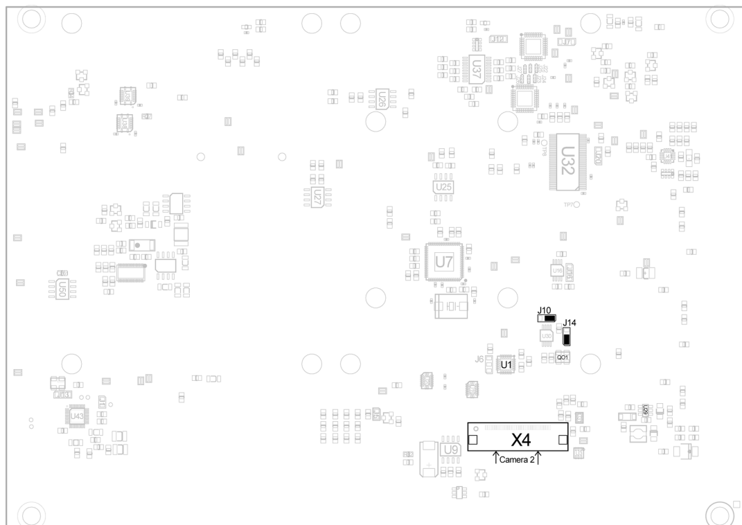
Figure 32: Camera Interfaces (bottom view)
