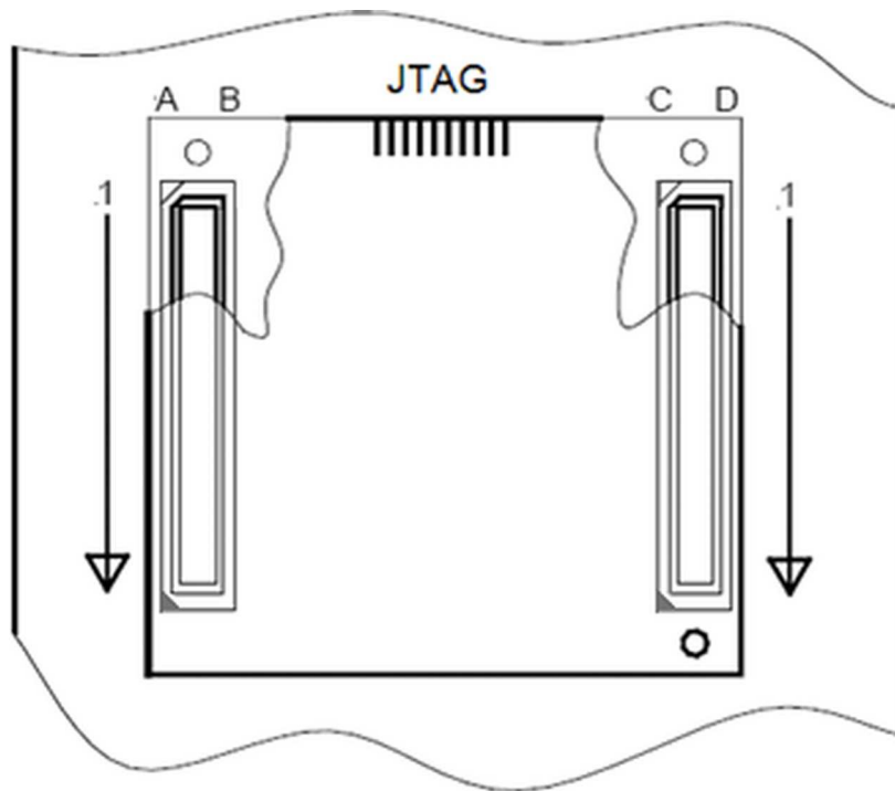
Figure 4: Pin-out of the phyCORE-Connector (top view, with cross section insert)
