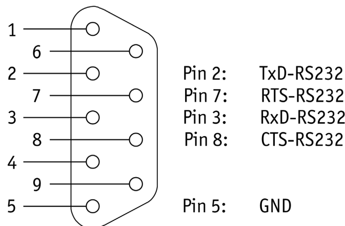
Figure 24: RS-232 connector P1 Signal Mapping
