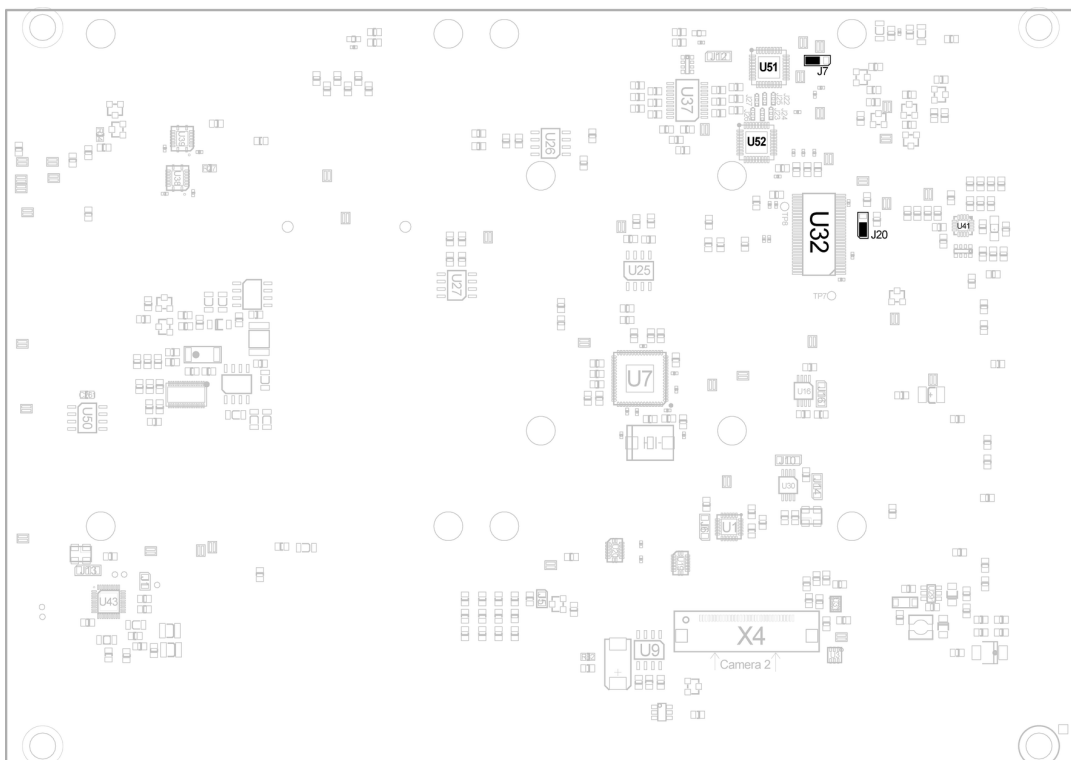
Figure 29: Display / Touch Connectivity (X12, X13)(bottom view)
