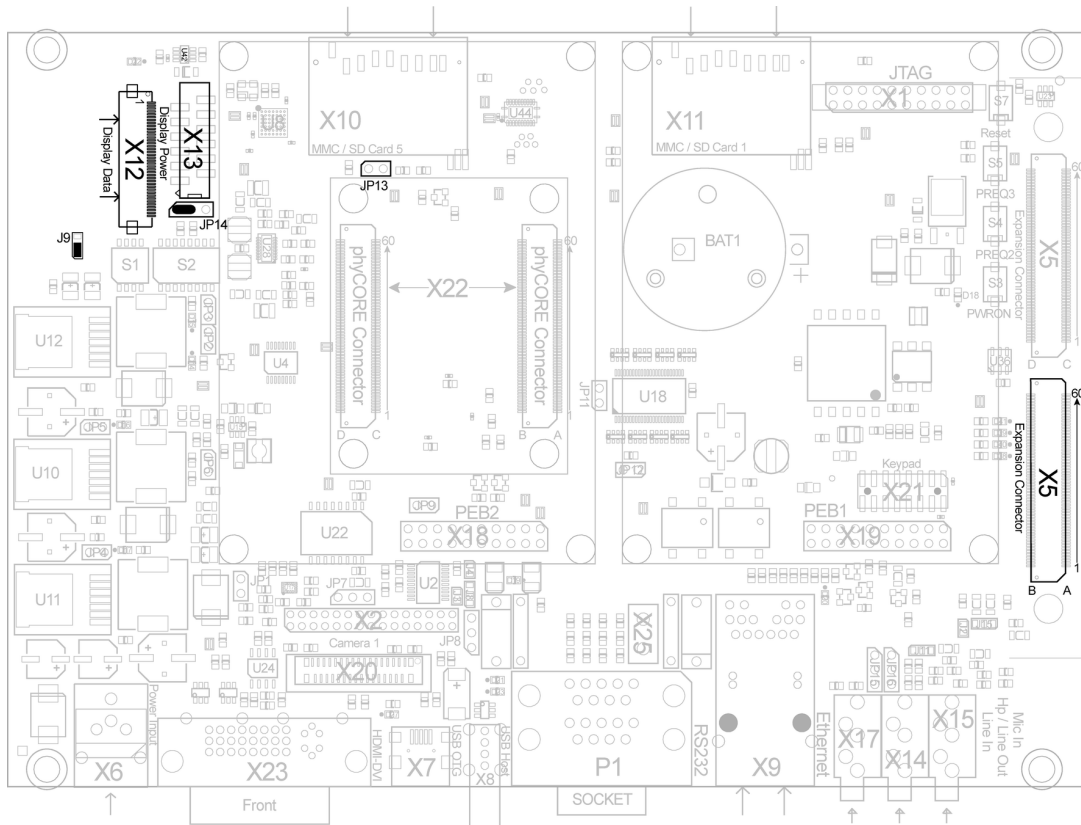
Figure 28: Display / Touch Connectivity (X12, X13)(top view)
