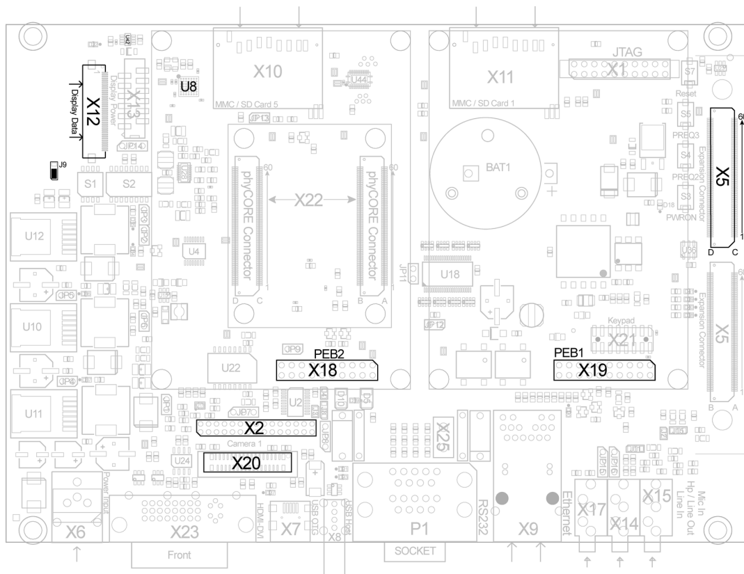
Figure 35: I 2 C Connectivity (top view)
