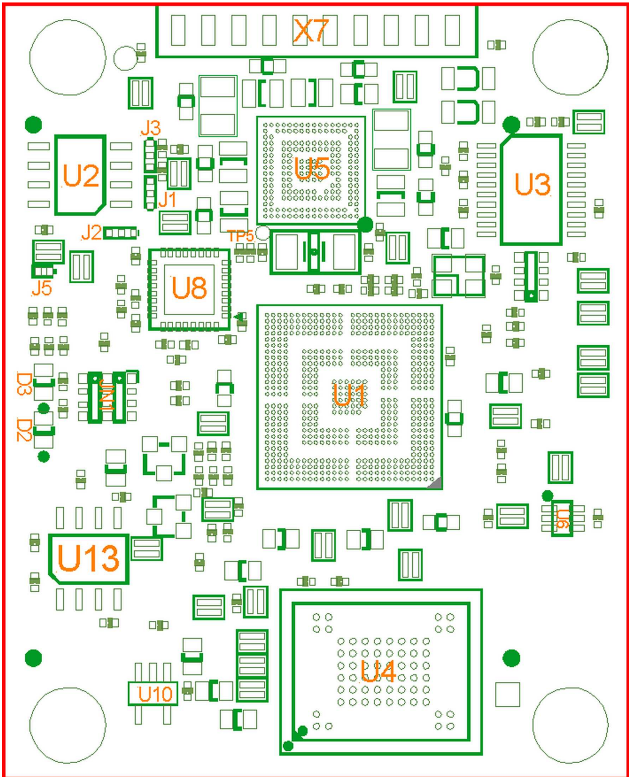
Figure 2: Top view of the phyCORE-OMAP44xx (controller side)
