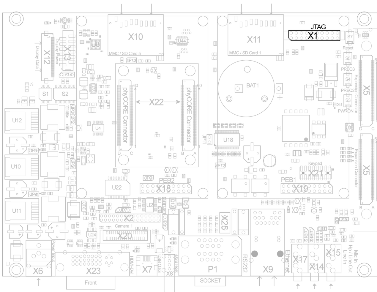
Figure 45: phyCORE JTAG Connectivity X1
