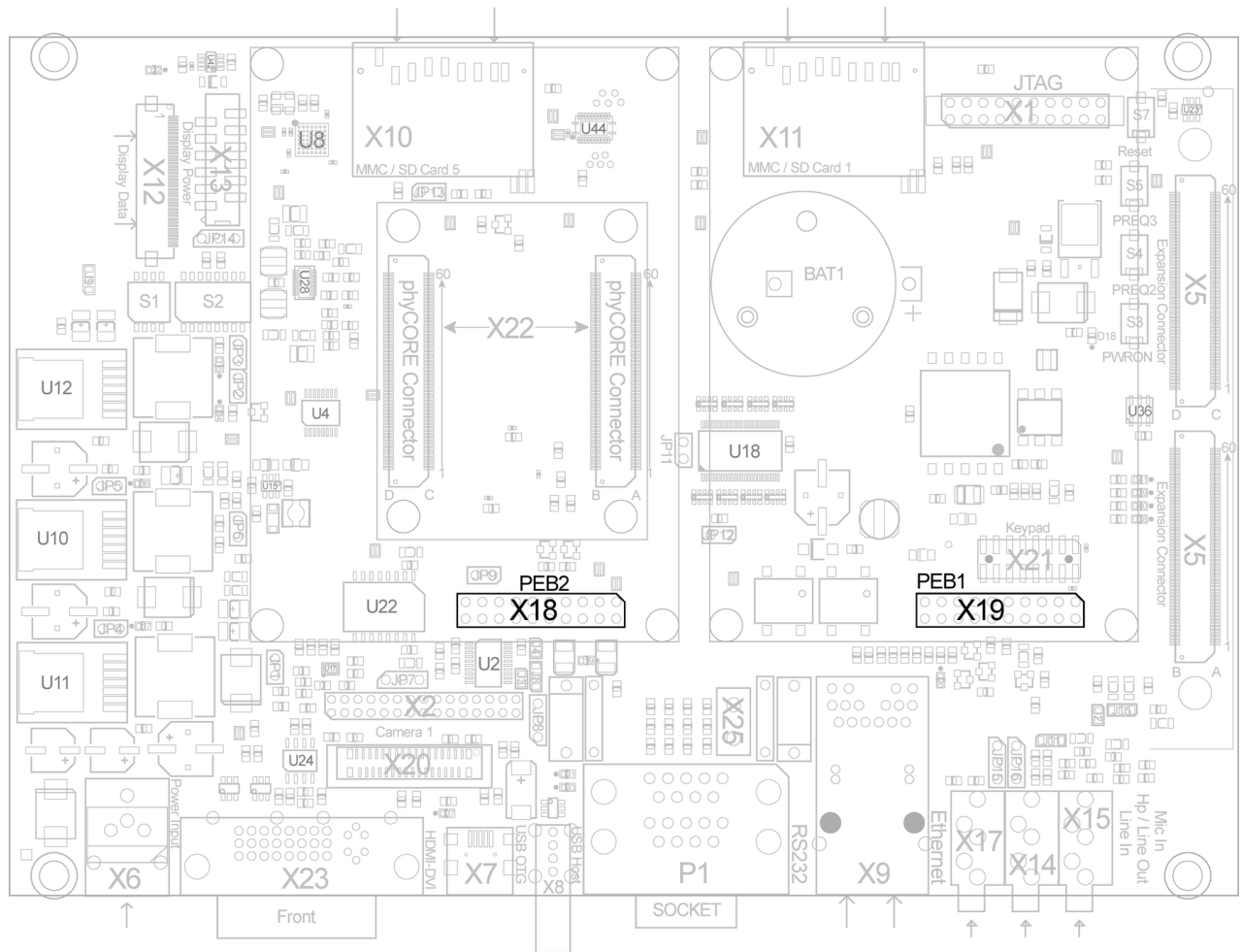
Figure 40: Extension Connectors X18, X19
