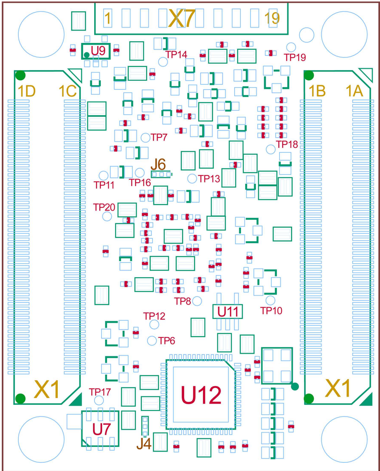
Figure 3: Bottom view of the phyCORE-OMAP44xx (connector side)
