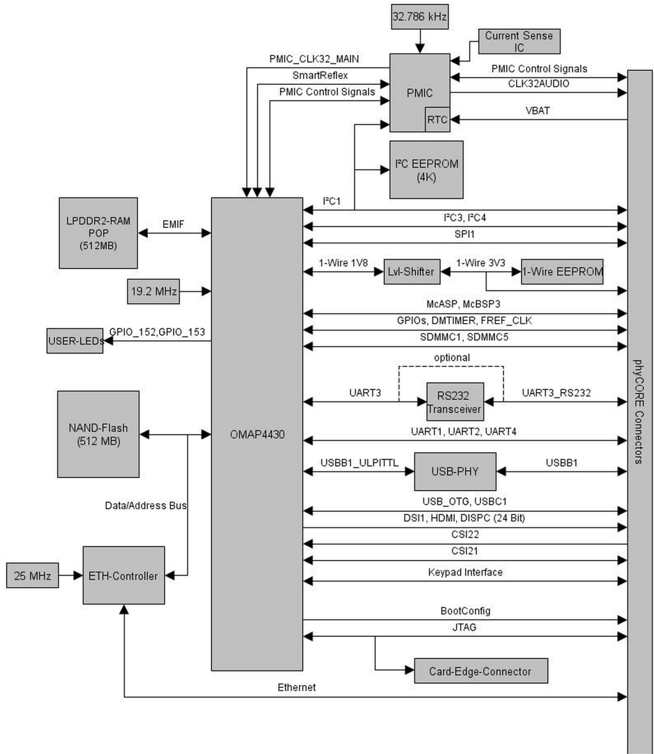
Figure 1: Block Diagram of the phyCORE-OMAP44xx
