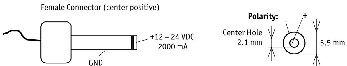
Figure 22: Power Connector Corresponding to Wall Adapter Input X6
