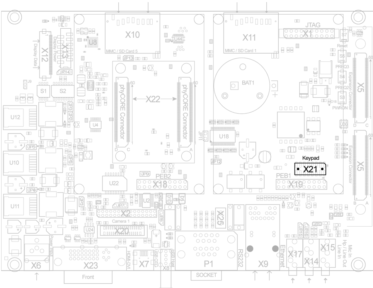
Figure 46: Keypad Connector X21
