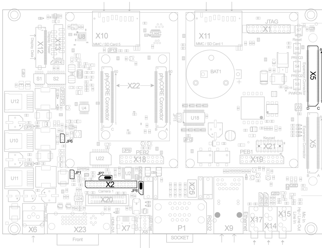
Figure 31: Camera Interfaces (top view)
