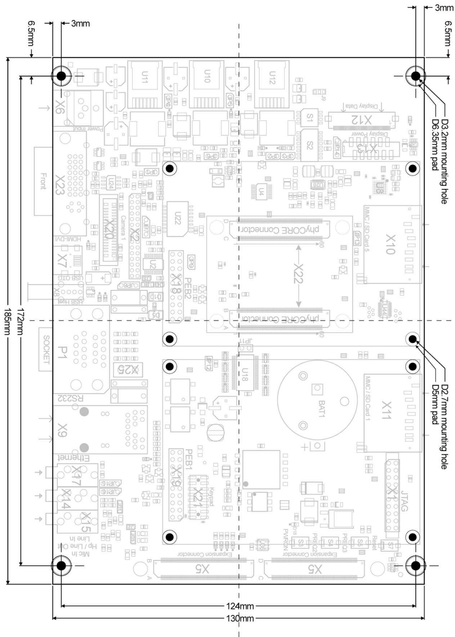
Figure 48: Carrier board physical dimensions
