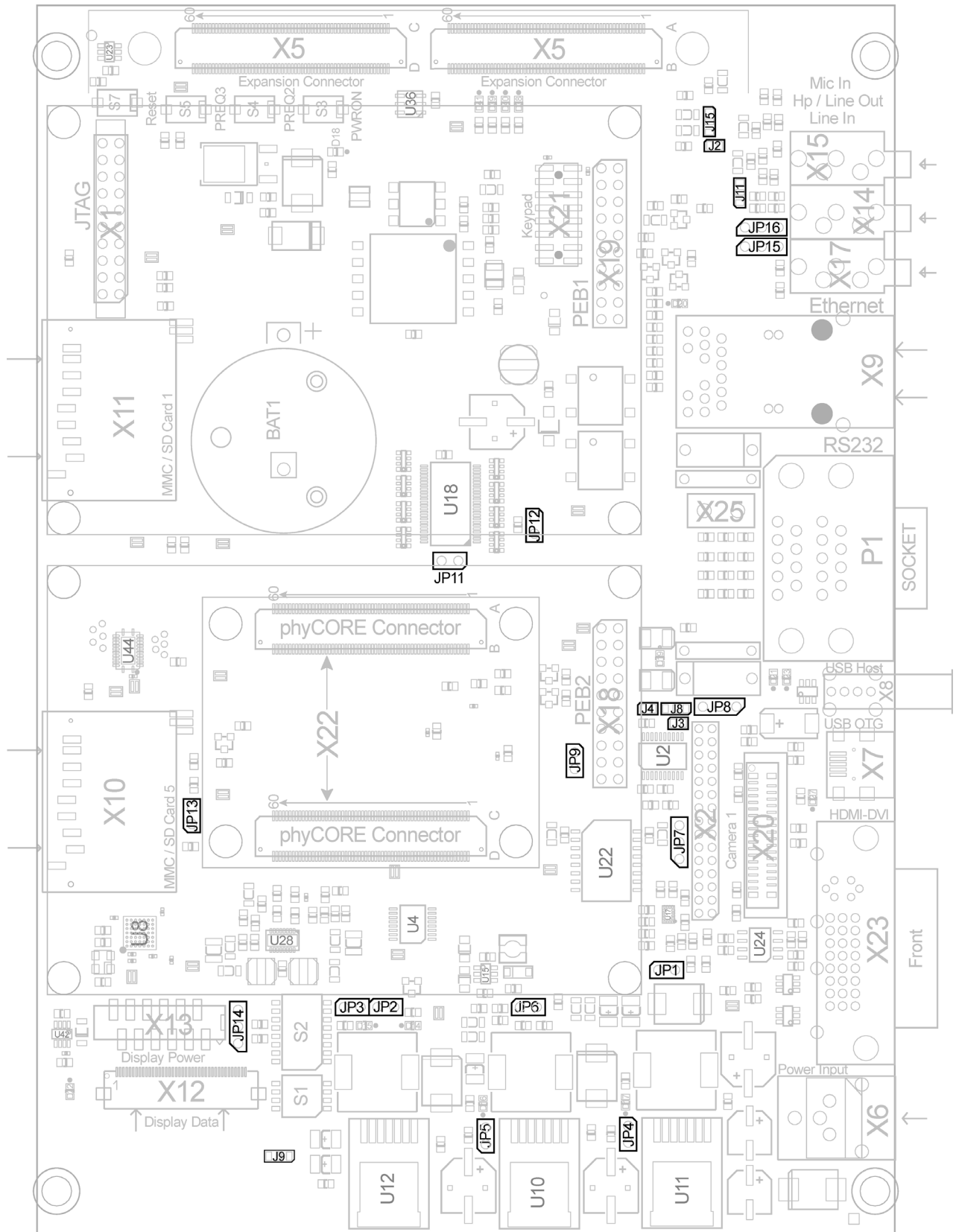
Figure 18: phyCORE-OMAP44xx Carrier Board Jumper Locations (top view)
