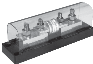
Figure 1a Fuse Block for Ring-lugged Battery Cables (TFBxxx)
