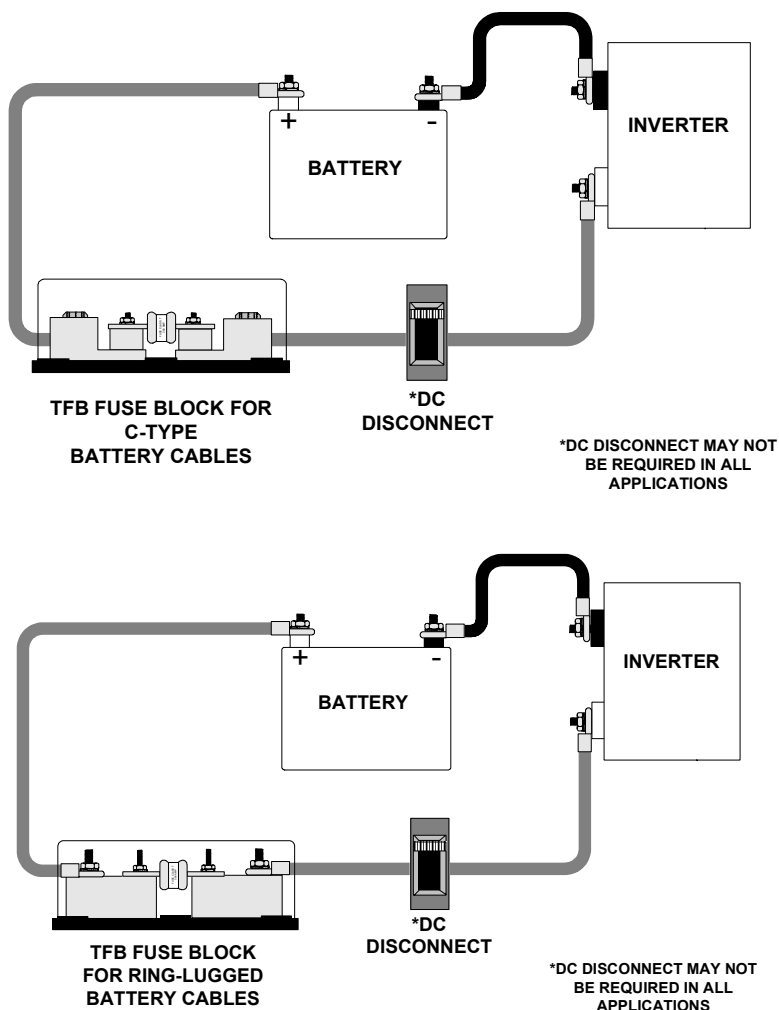
Figure 5 Wiring TFBs to the Battery, DC Disconnect, and Inverter
