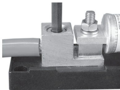
Figure 3 Installation for C-Type Battery Cables
