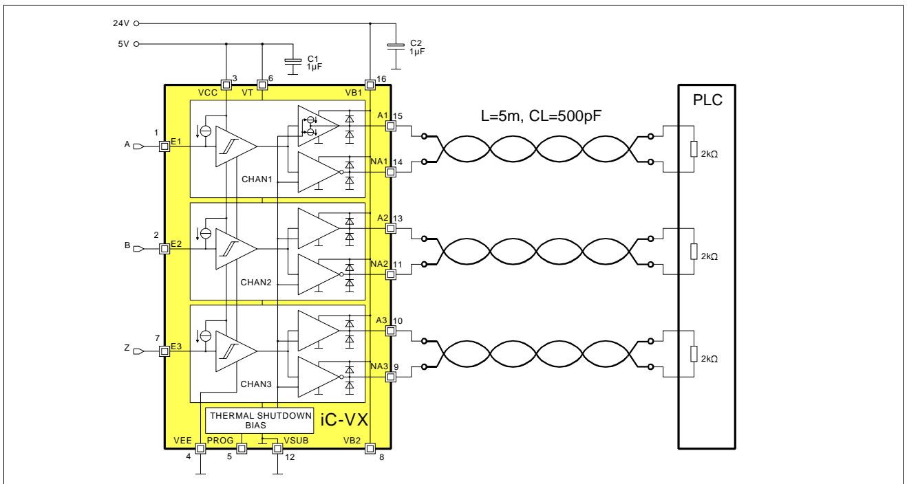
Fig. 1: Balanced data transmission at low capacitive load, PROG pin open: I(A) \geq 30mA
