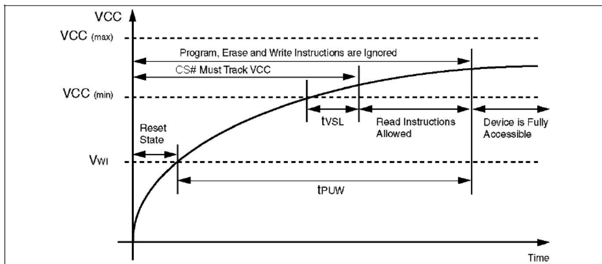
Figure 27. Power-up Timing
