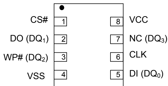
8 - LEAD VDFN
