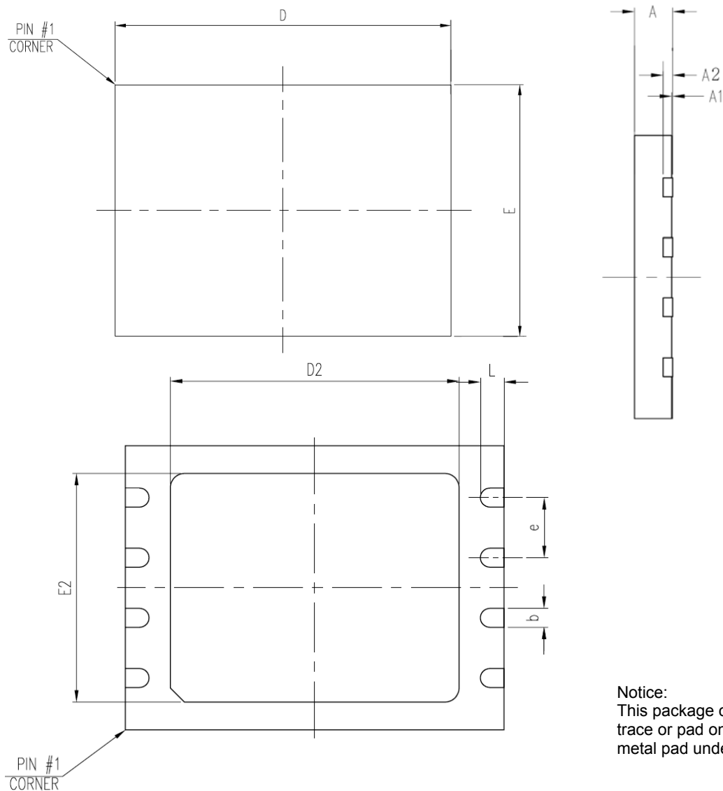
Figure 43. VDFN8 ( 5x6mm )
