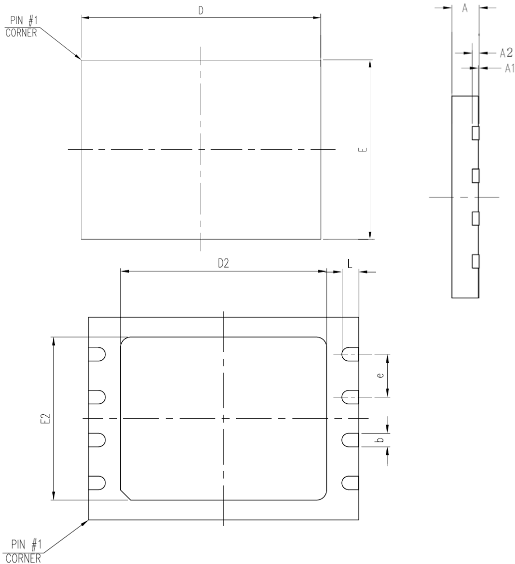
Figure 29. VDFN8 ( 5x6mm )
