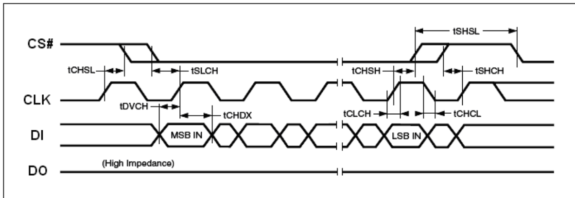
Figure 24. Input Timing
