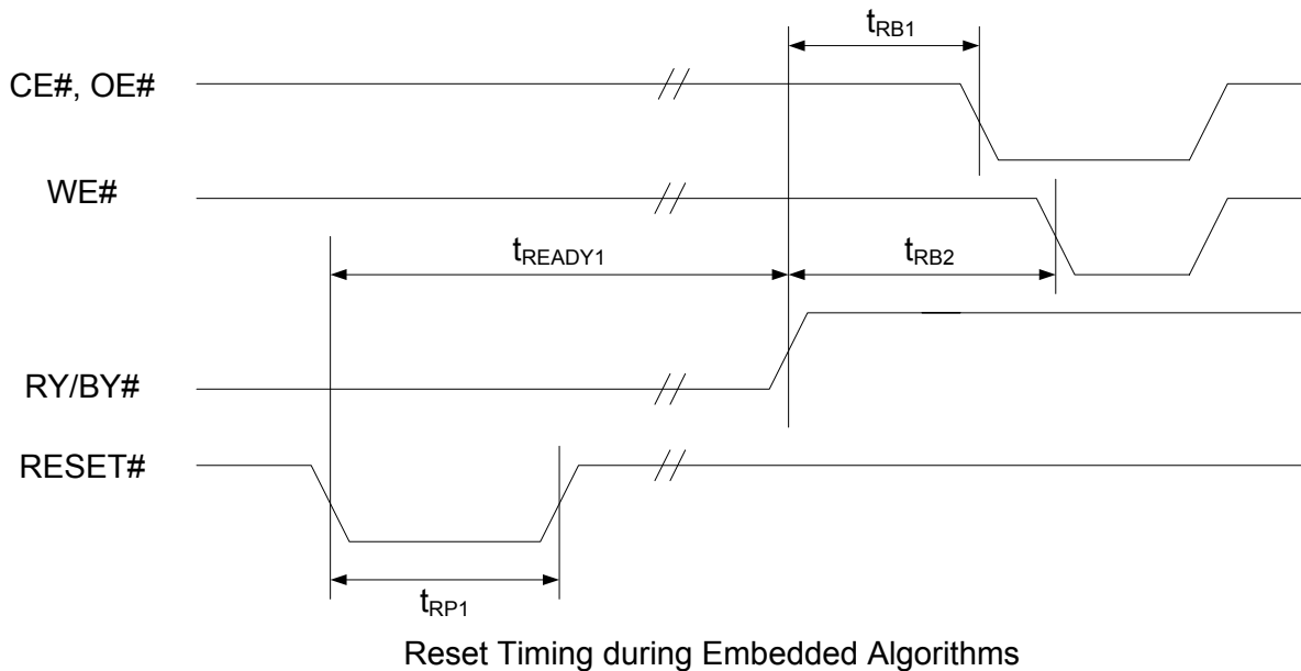
Figure 12. AC Waveforms for RESET# Reset# Timings
