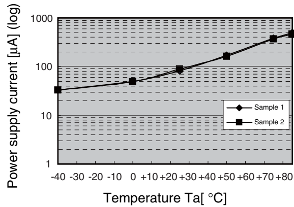
I_{CCT} temperature characteristics (semi-log) V_{CC} = 3.3\text{ V}
