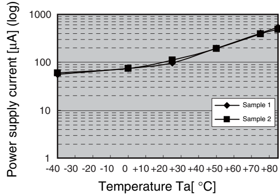
I_{CCL} temperature characteristics (semi-log) V_{CC} = 3.3\text{ V}
