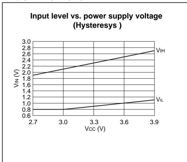
(4) "H" level input / "L" level input voltage (Hysteresis input)
