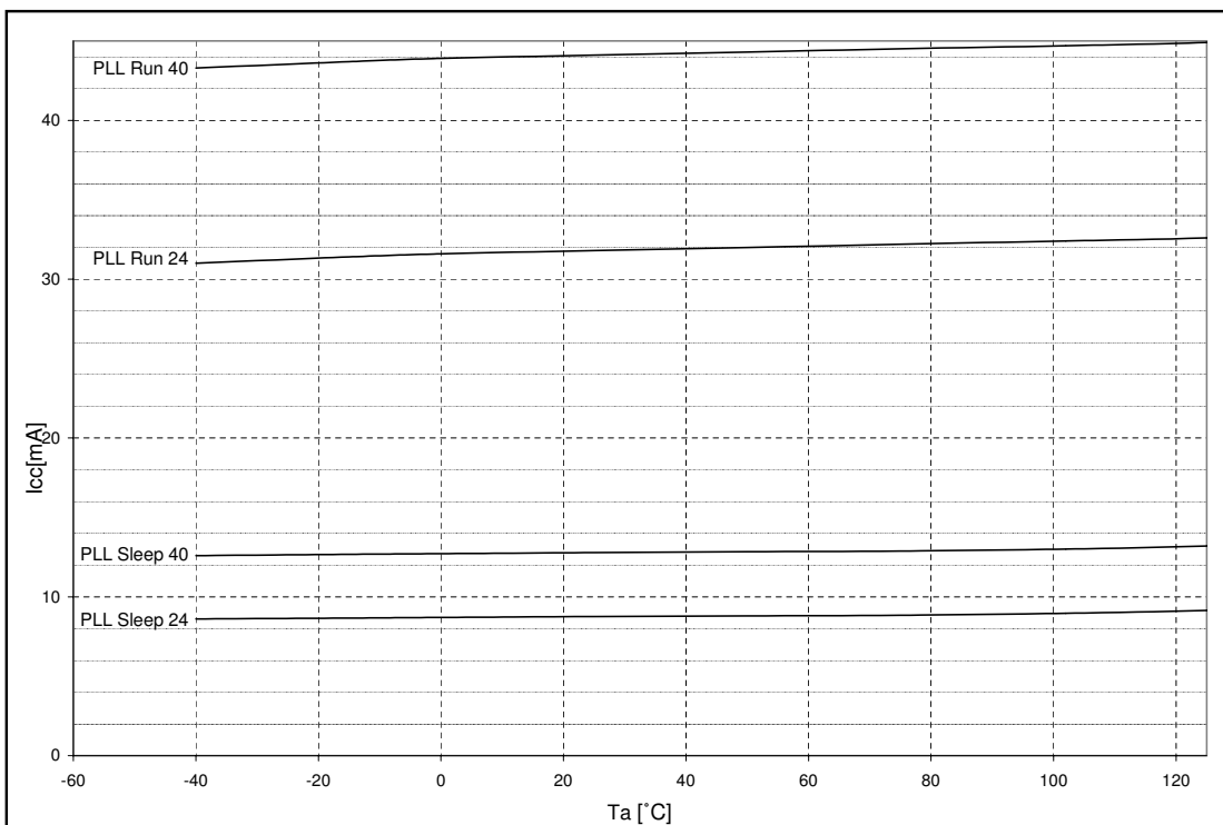
MB96F378/F379 PLL Run and Sleep mode currents
