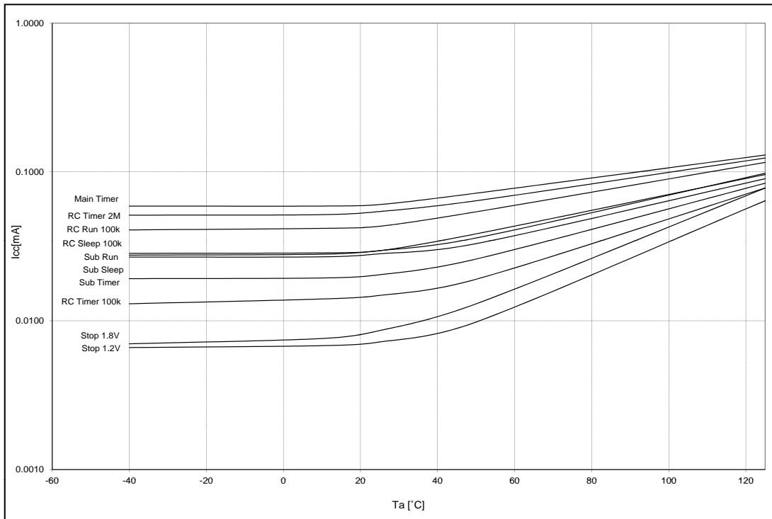
MB96375 Low power mode currents
