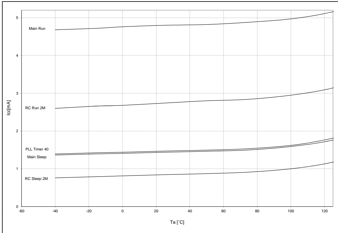
MB96F378/F379 Low power mode currents
