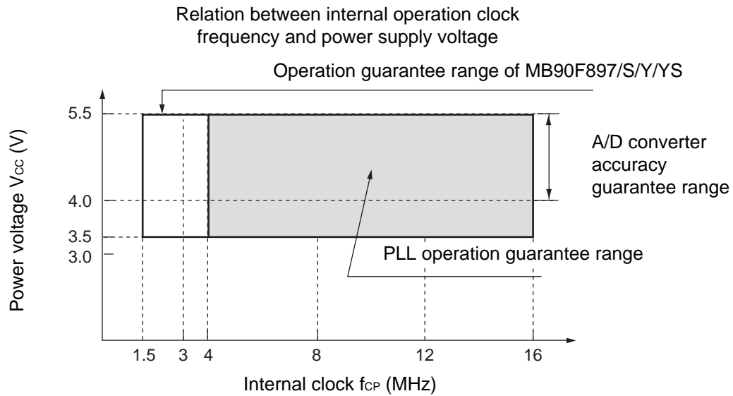
Relation among external clock frequency and internal clock frequency
