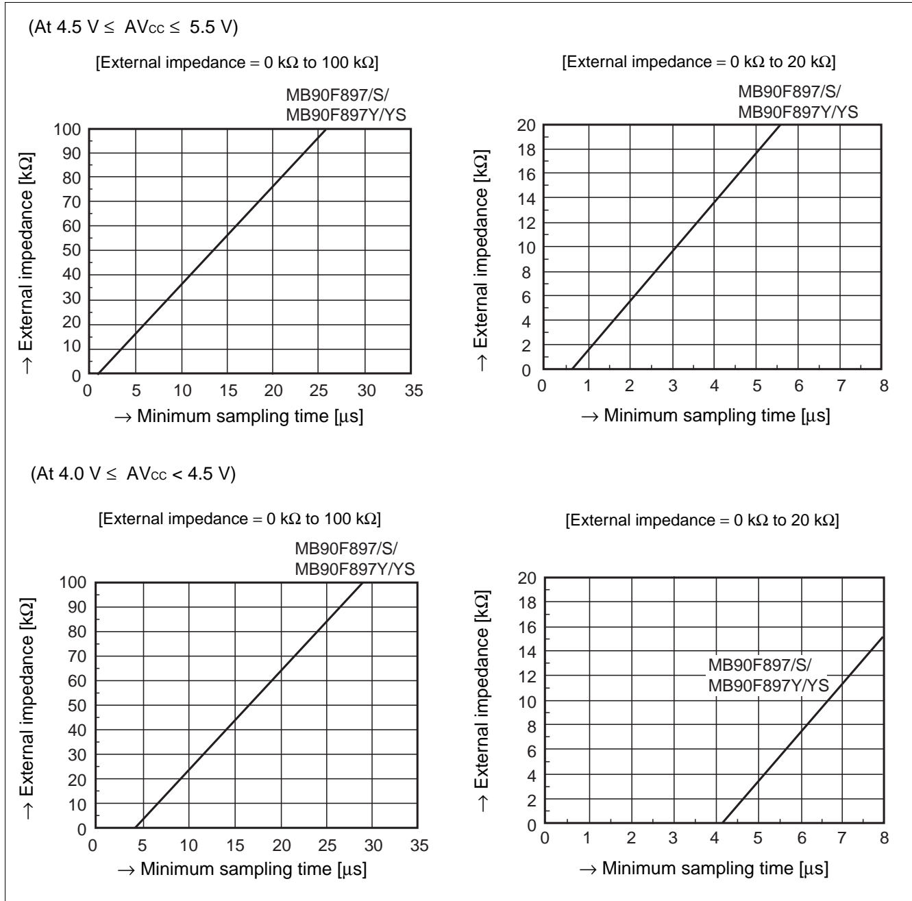
The relationship between the external impedance and minimum sampling time
