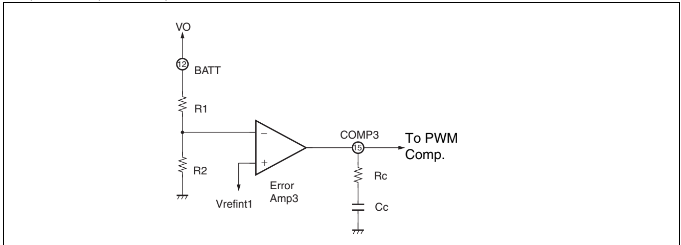
1pole-1zero phase compensation circuit
