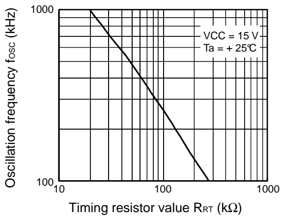
Oscillation frequency vs. Timing resistor value
