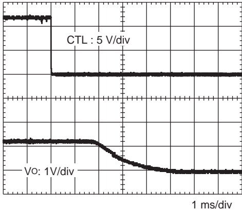
CTL Stop Waveform
