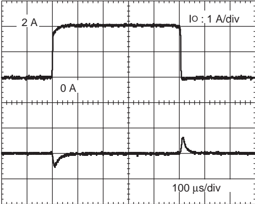
Load Sudden Change Waveform
