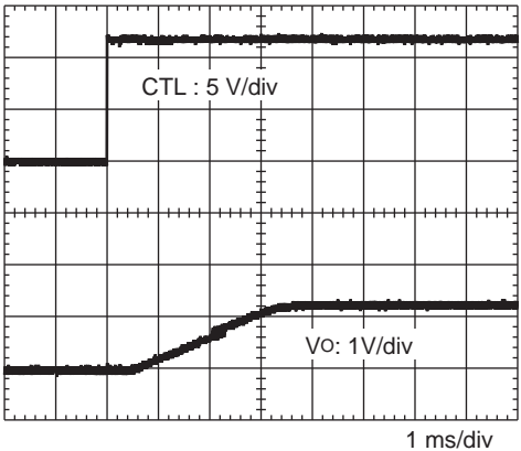
CTL Start-up Waveform
