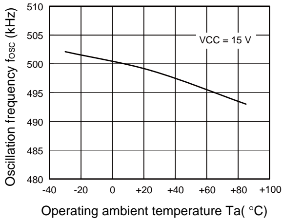
Oscillation frequency vs. Operating ambient temperature
