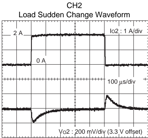
V_{IN} = 12\text{ V} , V_{o2} = 3.3\text{ V} I_{o2} = 0 \leftarrow \rightarrow 2\text{ A} , f_{osc} = 300\text{ kHz} , T_a = +25\text{ }^\circ\text{C}
