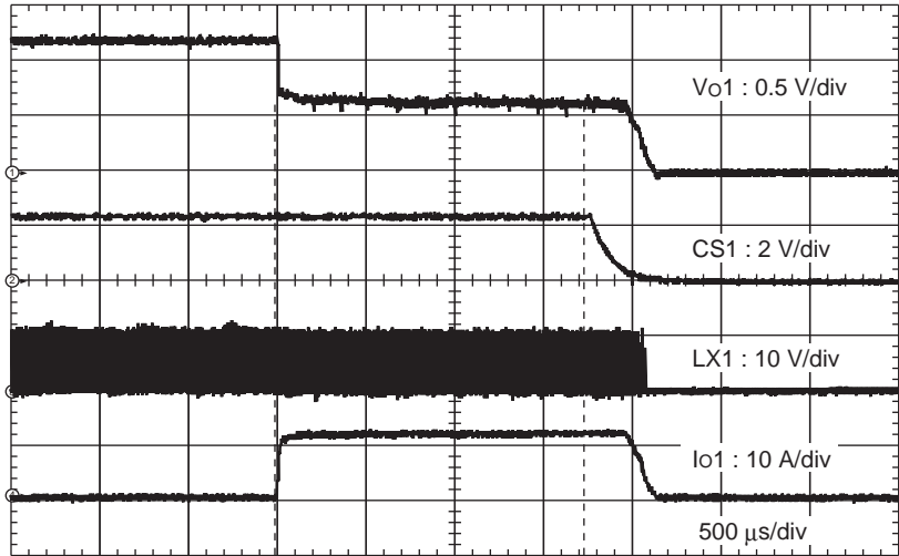
V_{IN} = 12\text{ V} , f_{osc} = 300\text{ kHz} , T_a = +25\text{ }^\circ\text{C} , Soft-start setting time = 3.0 ms V_{o1} = 1.2\text{ V} , I_{o1} = 5\text{ A} (0.24 \Omega ), V_{o2} = 3.3\text{ V} , I_{o2} = 5\text{ A} (0.66 \Omega )
