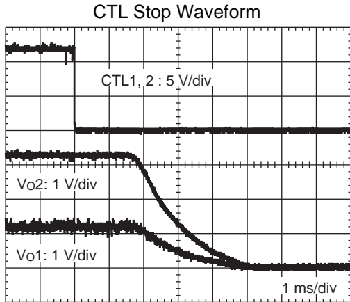
V_{IN} = 12\text{ V} , f_{osc} = 300\text{ kHz} , T_a = +25\text{ }^\circ\text{C} , Soft-start setting time = 3.0 ms V_{o1} = 1.2\text{ V} , I_{o1} = 5\text{ A} (0.24 \Omega ), V_{o2} = 3.3\text{ V} , I_{o2} = 5\text{ A} (0.66 \Omega )
