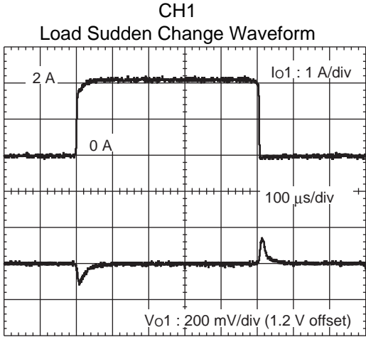
V_{IN} = 12\text{ V} , V_{o1} = 1.2\text{ V} I_{o1} = 0 \leftarrow \rightarrow 2\text{ A} , f_{osc} = 300\text{ kHz} , T_a = +25\text{ }^\circ\text{C}
