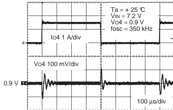
CH4 (fosc = 350 kHz, Vo4 = 0.9 V) Io4 = 0 A ↔ 1.5 A, Io4 slew rate = 1.5 A/μs
