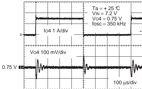
CH4 (fosc = 350 kHz, Vo4 = 0.75 V) Io4 = 0 A ↔ 1.5 A, Io4 slew rate = 1.5 A/μs
