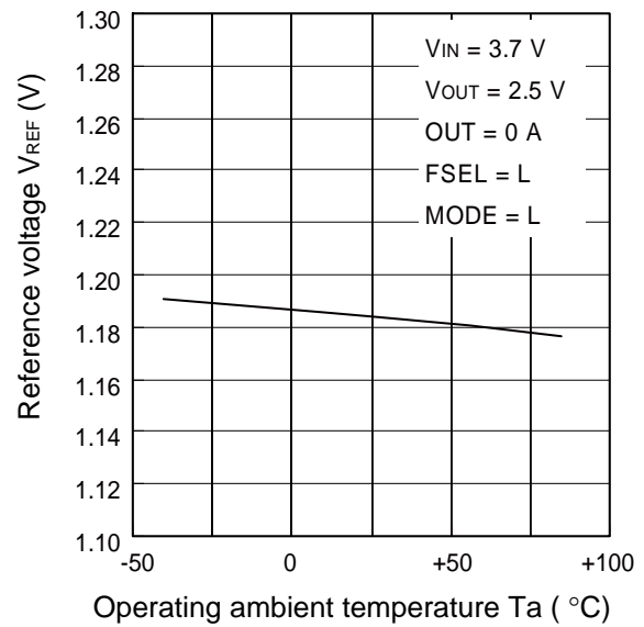
Reference voltage vs. Operating ambient temperature (2.0 MHz: PFM/PWM mode)
