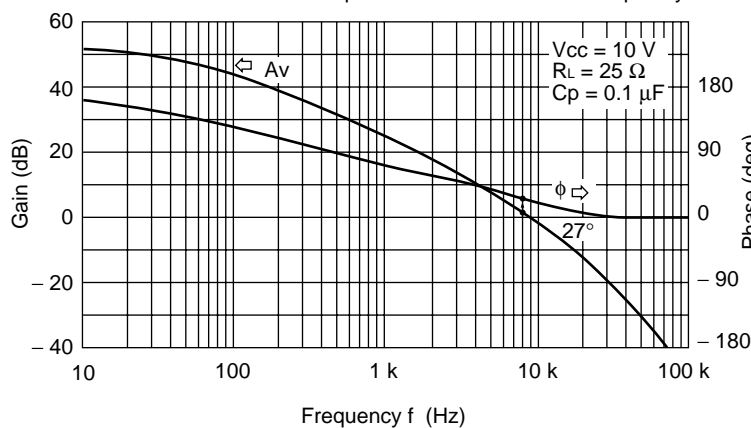
DC/DC converter + 5 V output Gain and Phase vs. Frequency
