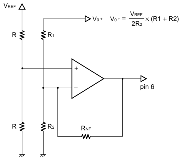
Figure 2 Error amp (channel 1) connection: Output voltage V_0 positive
