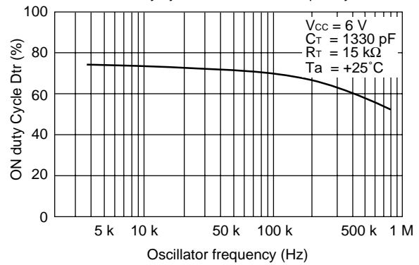
ON duty cycle vs. Oscillator frequency
