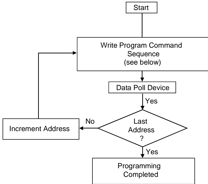
Program Command Sequence (Address /Command)
