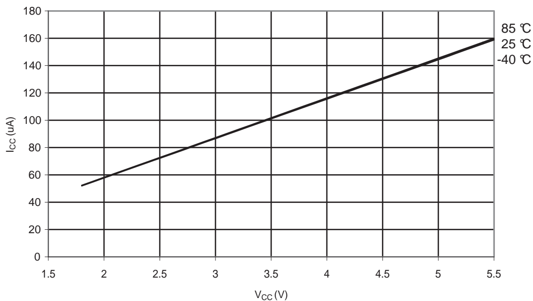
Figure 29-179. ATmega328P: AREF External Reference Current vs. V_{CC}
