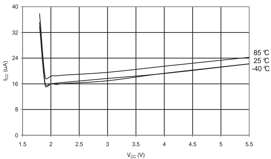
Figure 29-42. ATmega48PA: Brownout Detector Current vs. V_{CC}
