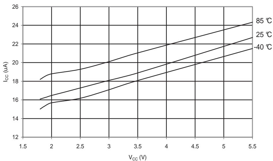
Figure 29-134. ATmega168PA: Brownout Detector Current vs. V_{CC}
