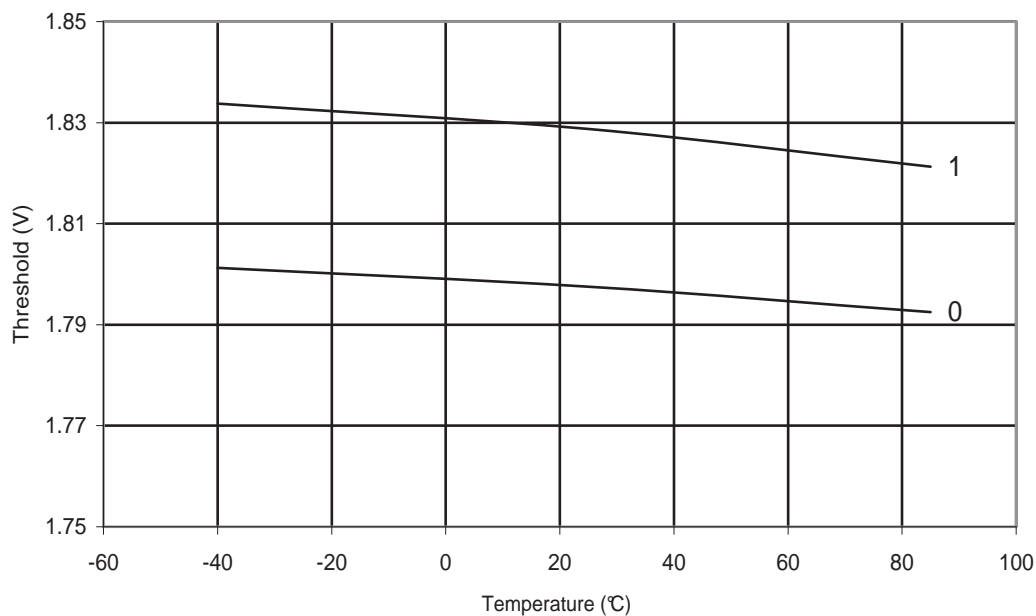
Figure 29-169. ATmega328P: BOD Thresholds vs. Temperature (BODLEVEL is 1.8 V)
