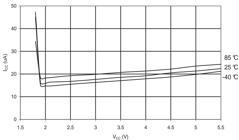
Figure 29-88. ATmega88PA: Brownout Detector Current vs. V_{CC}
