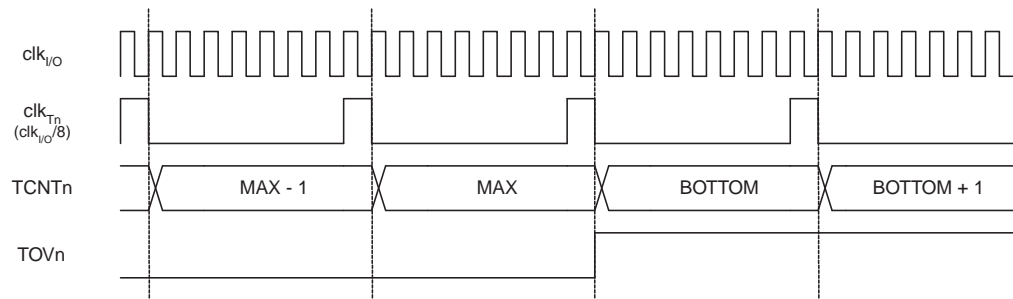
Figure 14-9. Timer/Counter Timing Diagram, with Prescaler ( f_{\text{clk}_{I/O}}/8 )
