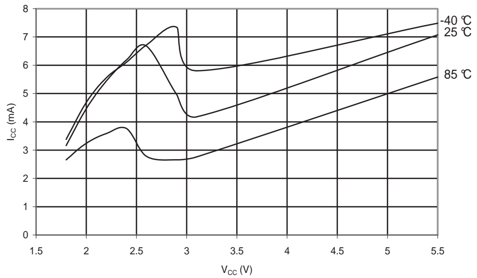
Figure 29-89. ATmega88PA: Programming Current vs. V_{CC}
