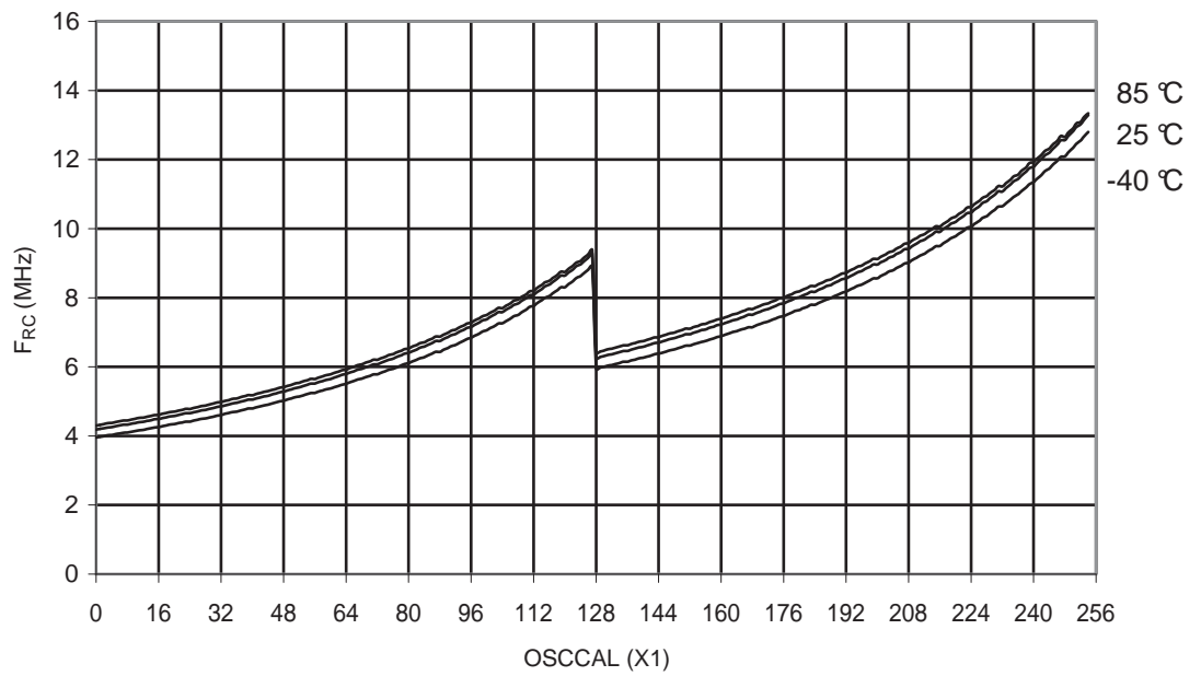
Figure 29-176. ATmega328P: Calibrated 8 MHz RC Oscillator Frequency vs. OSCCAL Value
