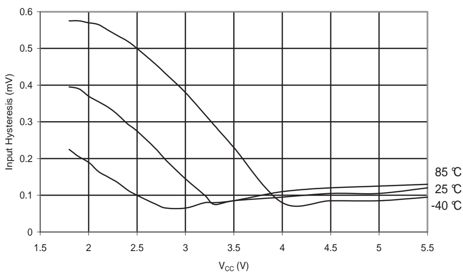
Figure 29-76. ATmega88PA: Reset Pin Input Hysteresis vs. V_{CC}
