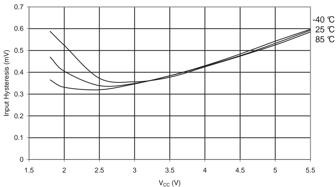
Figure 29-165. ATmega328P: I/O Pin Input Hysteresis vs. V_{CC}
