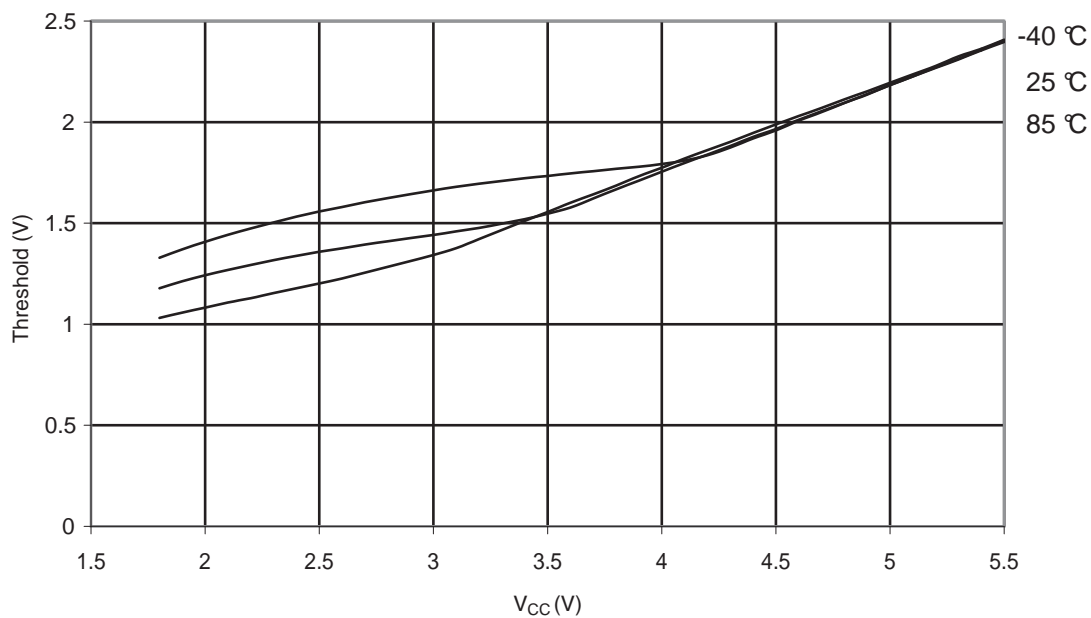
Figure 29-166. ATmega328P: Reset Input Threshold Voltage vs. V_{CC} ( V_{IH} , I/O Pin read as '1')
