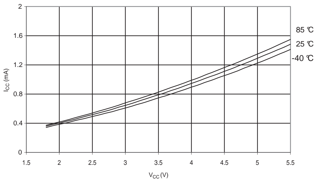
Figure 29-148. ATmega328P: Idle Supply Current vs. V_{CC} (Internal RC Oscillator, 8 MHz)
