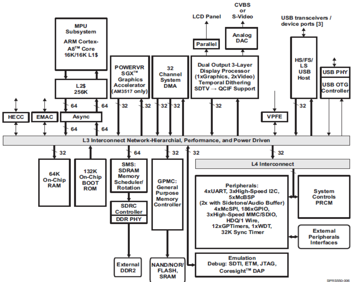
Figure 1-1. AM3517/05 Functional Block Diagram
